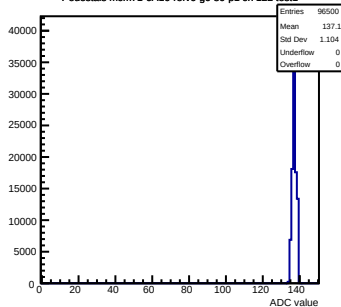
Pedestals mcm71-6A16-relv6-g0-s0-p1 ch 122 test1
