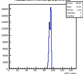
Pedestals mcm72-7C12-refv1-g0-s0-p1 ch 29 test1
