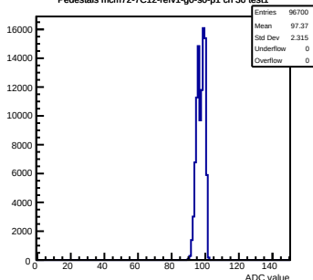
Pedestals mcm72-7C12-refv1-g0-s0-p1 ch 30 test1
