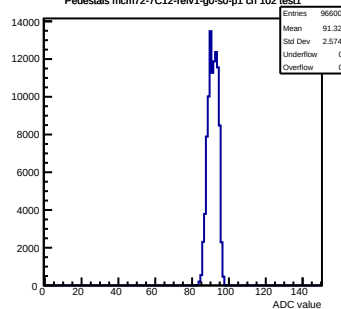
Pedestals mcm72-7C12-reV1-g0-s0-p1 ch 102 test1
