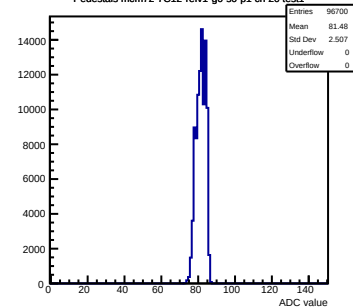
Pedestals mcm72-7C12-refv1-g0-s0-p1 ch 16 test1
