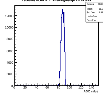
Pedestals mcm72-7C12-reV1-g0-s0-p1 ch 99 test1
