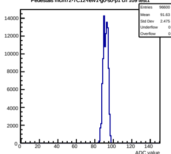
Pedestals mcm72-7C12-reV1-g0-s0-p1 ch 109 test1
