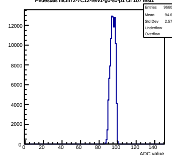
Pedestals mcm72-7C12-reV1-g0-s0-p1 ch 107 test1
