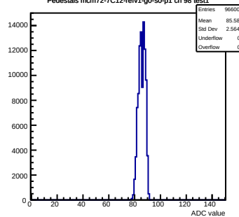
Pedestals mcm72-7C12-reV1-g0-s0-p1 ch 98 test1
