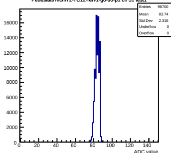
Pedestals mcm72-7C12-refv1-g0-s0-p1 ch 31 test1
