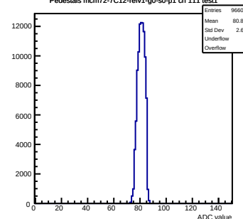
Pedestals mcm72-7C12-reV1-g0-s0-p1 ch 111 test1
