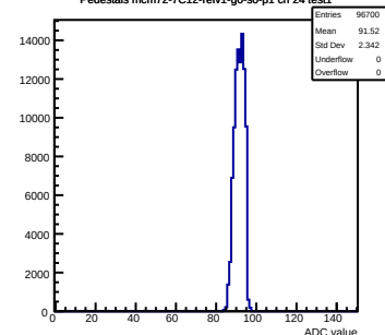
Pedestals mcm72-7C12-refv1-g0-s0-p1 ch 24 test1
