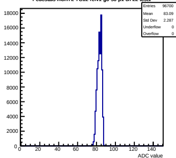
Pedestals mcm72-7C12-refv1-g0-s0-p1 ch 22 test1
