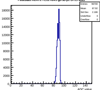
Pedestals mcm72-7C12-refv1-g0-s0-p1 ch 25 test1
