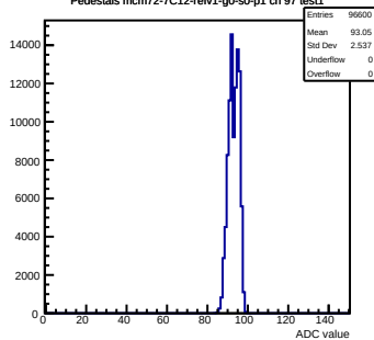
Pedestals mcm72-7C12-reV1-g0-s0-p1 ch 97 test1
