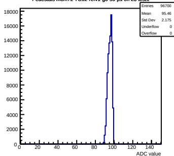
Pedestals mcm72-7C12-refv1-g0-s0-p1 ch 23 test1
