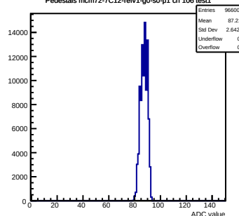
Pedestals mcm72-7C12-reV1-g0-s0-p1 ch 106 test1
