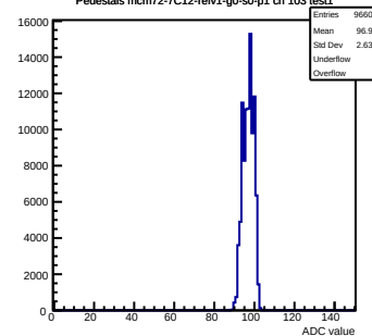
Pedestals mcm72-7C12-reV1-g0-s0-p1 ch 103 test1
