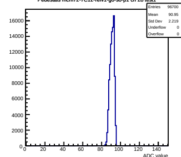
Pedestals mcm72-7C12-refv1-g0-s0-p1 ch 28 test1
