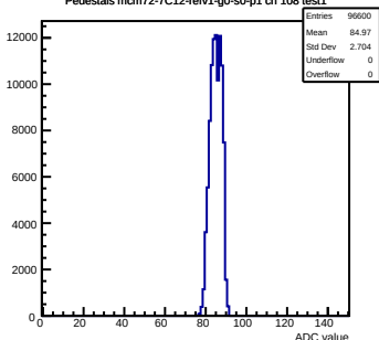
Pedestals mcm72-7C12-reV1-g0-s0-p1 ch 108 test1
