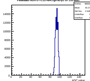
Pedestals mcm72-7C12-reV1-g0-s0-p1 ch 110 test1
