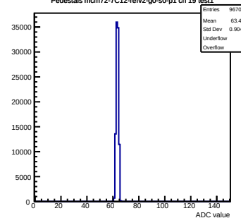
Pedestals mcm72-7C12-ref2-g0-s0-p1 ch 19 test1
