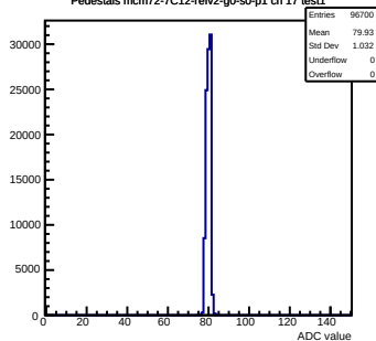
Pedestals mcm72-7C12-ref2-g0-s0-p1 ch 17 test1
