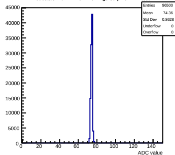
Pedestals mcm72-7C12-reV2-g0-s0-p1 ch 121 test1
