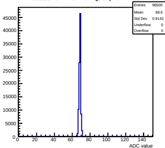
Pedestals mcm72-7C12-reV2-g0-s0-p1 ch 120 test1
