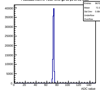
Pedestals mcm72-7C12-ref2-g0-s0-p1 ch 23 test1
