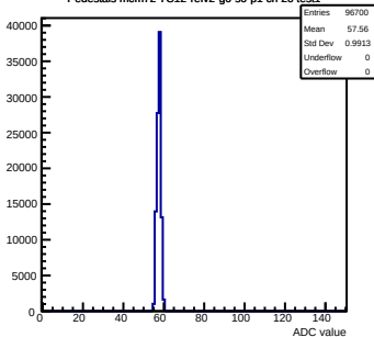
Pedestals mcm72-7C12-ref2-g0-s0-p1 ch 21 test1
