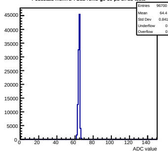
Pedestals mcm72-7C12-ref2-g0-s0-p1 ch 25 test1
