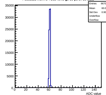
Pedestals mcm72-7C12-ref2-g0-s0-p1 ch 31 test1
