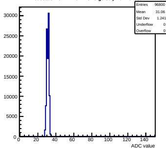
Pedestals mcm72-7C12-refv3-g0-s0-p1 ch 70 test1
