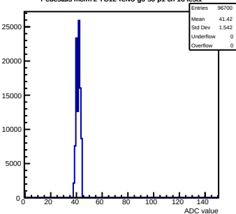
Pedestals mcm72-7C12-refv3-g0-s0-p1 ch 16 test1
