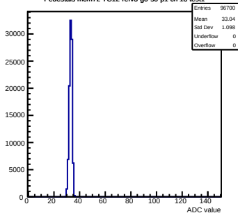
Pedestals mcm72-7C12-refv3-g0-s0-p1 ch 18 test1
