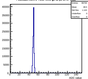
Pedestals mcm72-7C12-refv3-g0-s0-p1 ch 17 test1
