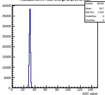
Pedestals mcm72-7C12-refv3-g0-s0-p1 ch 19 test1
