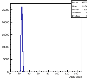
Pedestals mcm72-7C12-relv3-g0-s0-p1 ch 111 test1
