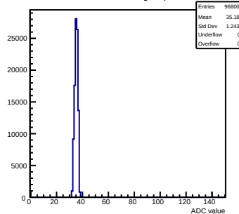
Pedestals mcm72-7C12-refv3-g0-s0-p1 ch 79 test1
