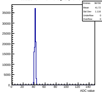
Pedestals mcm72-7C12-refv3-g0-s0-p1 ch 26 test1
