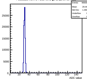
Pedestals mcm72-7C12-relv3-g0-s0-p1 ch 99 test1
