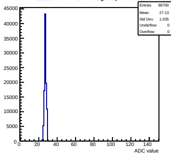
Pedestals mcm72-7C12-refv3-g0-s0-p1 ch 31 test1
