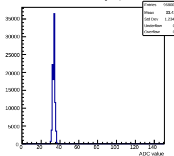
Pedestals mcm72-7C12-refv3-g0-s0-p1 ch 75 test1
