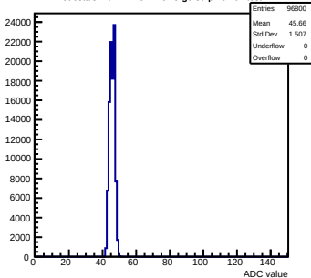
Pedestals mcm72-7C12-refv3-g0-s0-p1 ch 65 test1
