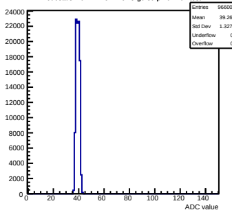
Pedestals mcm72-7C12-relv3-g0-s0-p1 ch 107 test1
