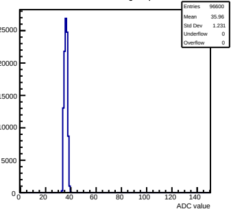
Pedestals mcm72-7C12-relv3-g0-s0-p1 ch 109 test1
