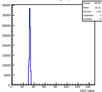
Pedestals mcm72-7C12-refv3-g0-s0-p1 ch 27 test1
