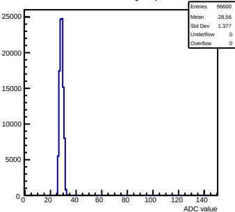
Pedestals mcm72-7C12-relv3-g0-s0-p1 ch 108 test1
