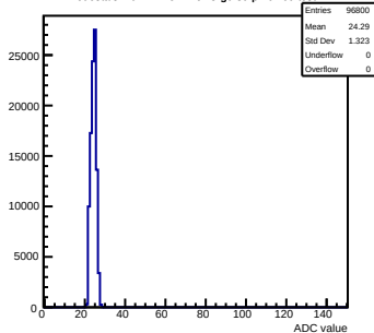
Pedestals mcm72-7C12-refv3-g0-s0-p1 ch 69 test1
