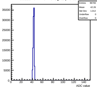
Pedestals mcm72-7C12-refv3-g0-s0-p1 ch 30 test1
