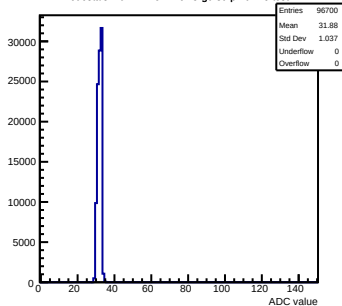
Pedestals mcm72-7C12-refv3-g0-s0-p1 ch 25 test1
