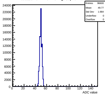
Pedestals mcm72-7C12-refV4-g0-s0-p1 ch 106 test1
