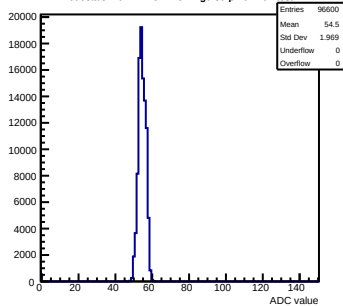
Pedestals mcm72-7C12-refV4-g0-s0-p1 ch 102 test1
