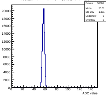
Pedestals mcm72-7C12-refV4-g0-s0-p1 ch 97 test1
