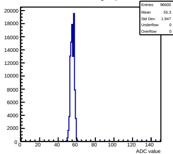
Pedestals mcm72-7C12-refV4-g0-s0-p1 ch 110 test1
