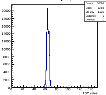
Pedestals mcm72-7C12-refV4-g0-s0-p1 ch 104 test1
