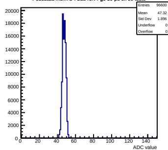
Pedestals mcm72-7C12-refV4-g0-s0-p1 ch 99 test1
