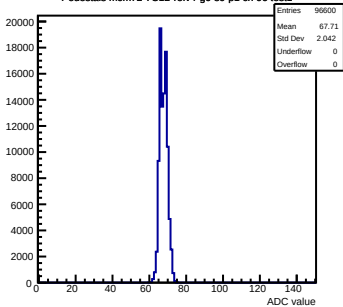
Pedestals mcm72-7C12-refV4-g0-s0-p1 ch 96 test1
