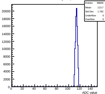
Pedestals mcm72-7C12-refv6-g0-s0-p1 ch 40 test1
