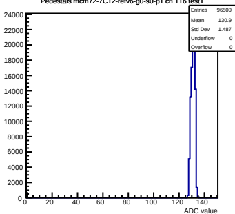
Pedestals mcm72-7C12-relv6-g0-s0-p1 ch 116 test1
