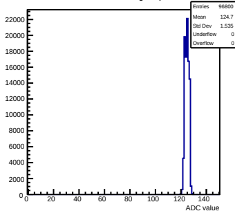
Pedestals mcm72-7C12-refv6-g0-s0-p1 ch 79 test1
