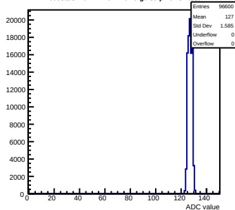
Pedestals mcm72-7C12-refv6-g0-s0-p1 ch 37 test1
