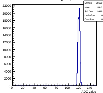
Pedestals mcm72-7C12-refv6-g0-s0-p1 ch 38 test1
