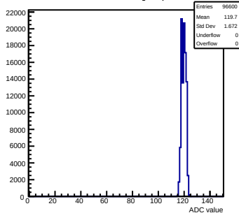
Pedestals mcm72-7C12-refv6-g0-s0-p1 ch 43 test1
