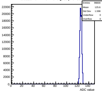
Pedestals mcm72-7C12-refv6-g0-s0-p1 ch 36 test1
