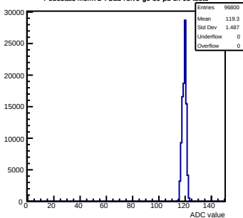
Pedestals mcm72-7C12-refv6-g0-s0-p1 ch 65 test1
