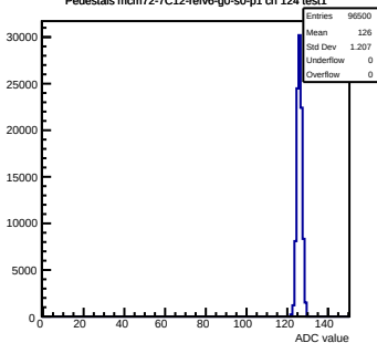
Pedestals mcm72-7C12-relv6-g0-s0-p1 ch 124 test1
