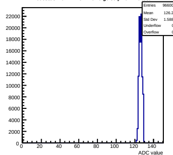
Pedestals mcm72-7C12-relv6-g0-s0-p1 ch 110 test1
