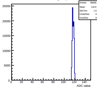
Pedestals mcm72-7C12-refv6-g0-s0-p1 ch 47 test1
