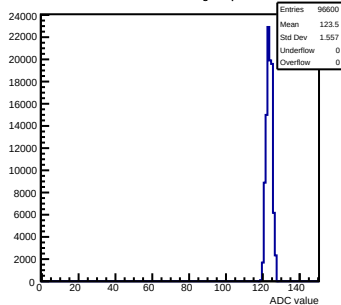
Pedestals mcm72-7C12-refv6-g0-s0-p1 ch 41 test1
