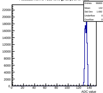
Pedestals mcm72-7C12-refv6-g0-s0-p1 ch 67 test1
