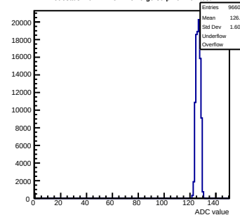
Pedestals mcm72-7C12-relv6-g0-s0-p1 ch 107 test1
