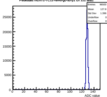
Pedestals mcm72-7C12-relv6-g0-s0-p1 ch 122 test1
