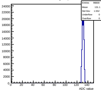
Pedestals mcm72-7C12-refv6-g0-s0-p1 ch 44 test1
