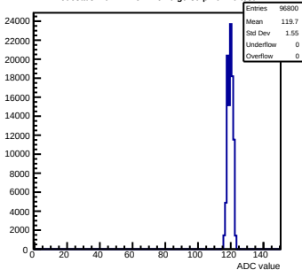
Pedestals mcm72-7C12-refv6-g0-s0-p1 ch 70 test1
