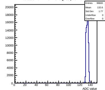
Pedestals mcm72-7C12-relv6-g0-s0-p1 ch 104 test1
