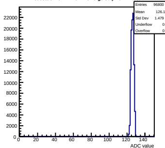
Pedestals mcm72-7C12-refv6-g0-s0-p1 ch 71 test1
