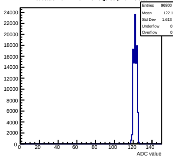
Pedestals mcm72-7C12-refv6-g0-s0-p1 ch 75 test1
