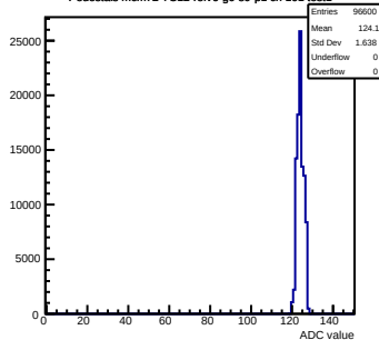
Pedestals mcm72-7C12-relv6-g0-s0-p1 ch 101 test1
