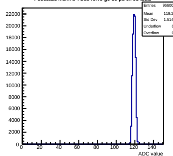
Pedestals mcm72-7C12-relv6-g0-s0-p1 ch 98 test1
