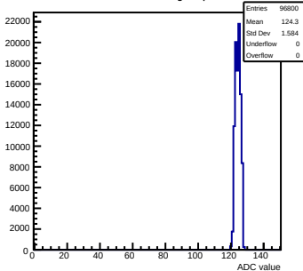
Pedestals mcm72-7C12-refv6-g0-s0-p1 ch 76 test1
