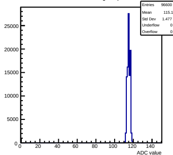
Pedestals mcm72-7C12-refv6-g0-s0-p1 ch 46 test1
