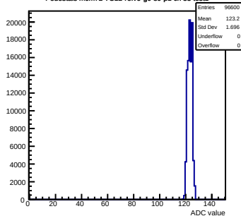
Pedestals mcm72-7C12-refv6-g0-s0-p1 ch 33 test1
