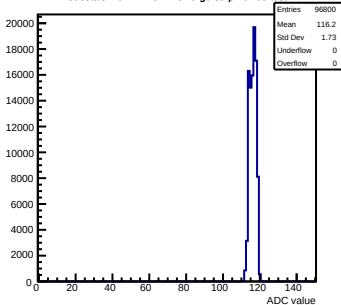
Pedestals mcm72-7C12-refv6-g0-s0-p1 ch 69 test1
