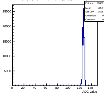
Pedestals mcm72-7C12-refv6-g0-s0-p1 ch 34 test1
