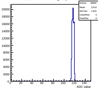
Pedestals mcm72-7C12-refv6-g0-s0-p1 ch 73 test1
