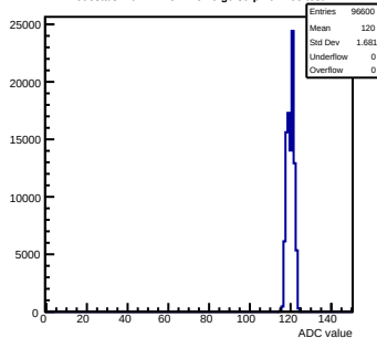
Pedestals mcm72-7C12-relv6-g0-s0-p1 ch 105 test1
