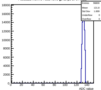
Pedestals mcm72-7C12-refv6-g0-s0-p1 ch 64 test1
