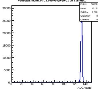
Pedestals mcm72-7C12-relv6-g0-s0-p1 ch 118 test1
