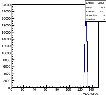
Pedestals mcm72-7C12-refv6-g0-s0-p1 ch 77 test1
