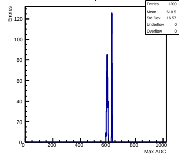
Max mcm 0 chip 7 chan 2 test1
