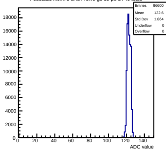
Pedestals mcm73-2A14-refV0-g0-s0-p1 ch 40 test1
