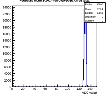
Pedestals mcm73-2A14-refv0-g0-s0-p1 ch 65 test1
