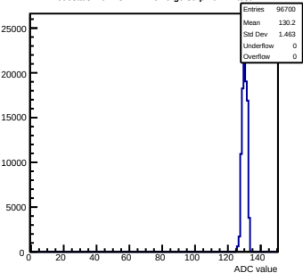
Pedestals mcm73-2A14-refV0-g0-s0-p1 ch 27 test1
