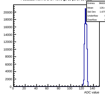
Pedestals mcm73-2A14-refV0-g0-s0-p1 ch 38 test1
