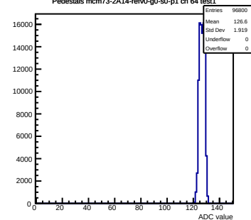
Pedestals mcm73-2A14-refv0-g0-s0-p1 ch 64 test1
