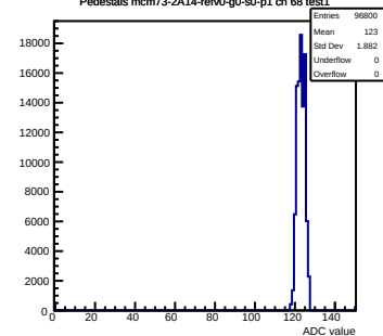
Pedestals mcm73-2A14-refv0-g0-s0-p1 ch 68 test1
