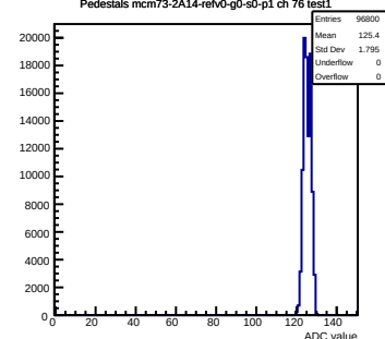
Pedestals mcm73-2A14-refv0-g0-s0-p1 ch 76 test1
