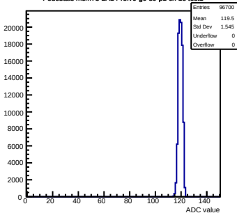
Pedestals mcm73-2A14-refV0-g0-s0-p1 ch 18 test1
