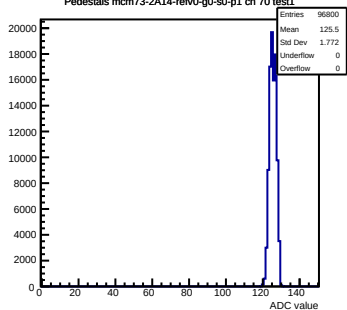
Pedestals mcm73-2A14-refv0-g0-s0-p1 ch 70 test1
