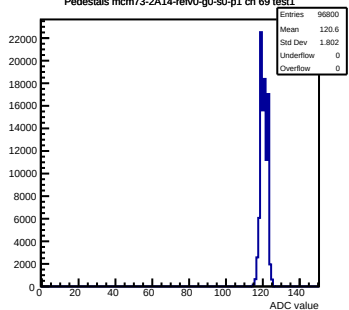
Pedestals mcm73-2A14-refv0-g0-s0-p1 ch 69 test1
