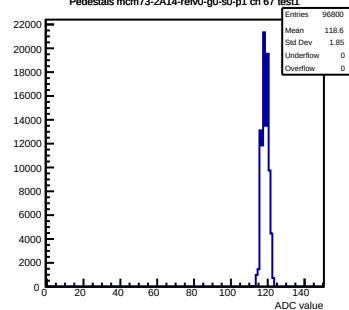
Pedestals mcm73-2A14-refv0-g0-s0-p1 ch 67 test1
