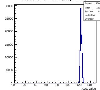
Pedestals mcm73-2A14-refV0-g0-s0-p1 ch 47 test1
