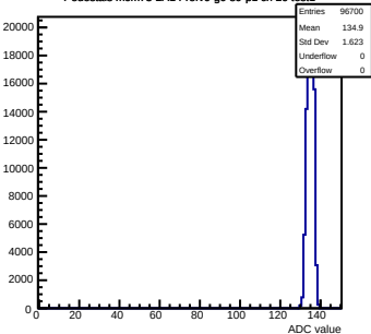
Pedestals mcm73-2A14-refV0-g0-s0-p1 ch 20 test1
