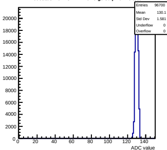
Pedestals mcm73-2A14-refV0-g0-s0-p1 ch 26 test1
