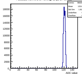
Pedestals mcm73-2A14-refV0-g0-s0-p1 ch 42 test1
