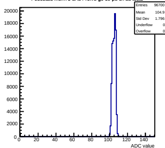
Pedestals mcm73-2A14-refv1-q0-s0-p1 ch 22 test1
