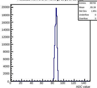
Pedestals mcm73-2A14-refv1-q0-s0-p1 ch 21 test1
