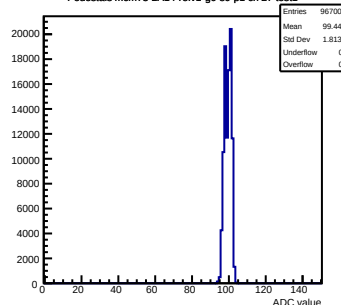
Pedestals mcm73-2A14-refv1-q0-s0-p1 ch 27 test1
