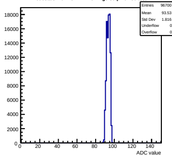
Pedestals mcm73-2A14-refv1-q0-s0-p1 ch 30 test1
