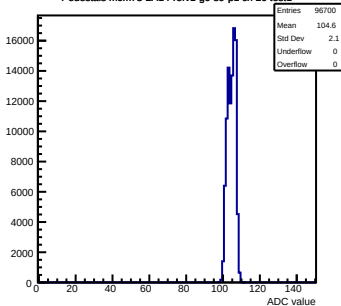
Pedestals mcm73-2A14-refv1-q0-s0-p1 ch 20 test1
