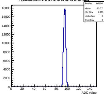
Pedestals mcm73-2A14-refv1-q0-s0-p1 ch 17 test1
