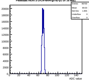
Pedestals mcm73-2A14-refv4-g0-s0-p1 ch 16 test1
