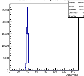
Pedestals mcm73-2A14-refv4-g0-s0-p1 ch 98 test1
