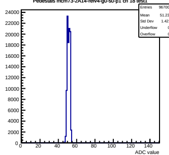
Pedestals mcm73-2A14-refv4-g0-s0-p1 ch 18 test1
