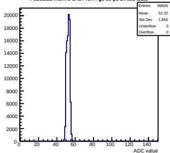
Pedestals mcm73-2A14-refv4-g0-s0-p1 ch 105 test1
