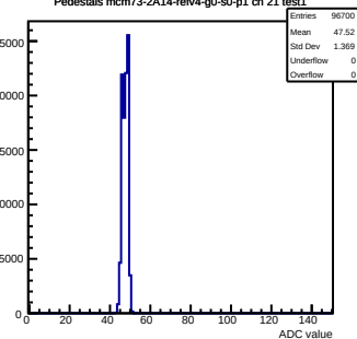
Pedestals mcm73-2A14-refv4-g0-s0-p1 ch 21 test1
