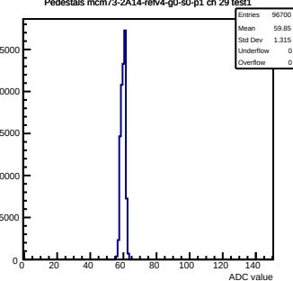
Pedestals mcm73-2A14-refv4-g0-s0-p1 ch 29 test1
