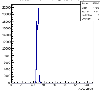
Pedestals mcm73-2A14-refv4-g0-s0-p1 ch 109 test1
