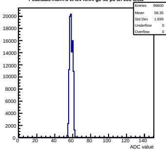
Pedestals mcm73-2A14-refv4-g0-s0-p1 ch 100 test1
