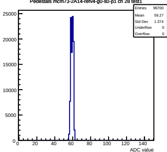
Pedestals mcm73-2A14-refv4-g0-s0-p1 ch 28 test1
