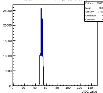
Pedestals mcm73-2A14-refv4-g0-s0-p1 ch 99 test1
