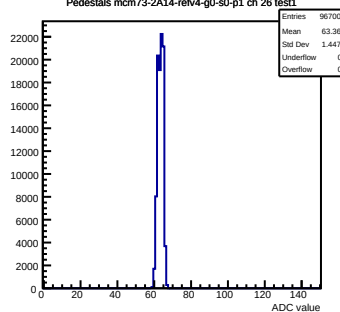
Pedestals mcm73-2A14-refv4-g0-s0-p1 ch 26 test1
