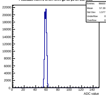
Pedestals mcm73-2A14-refv4-g0-s0-p1 ch 102 test1
