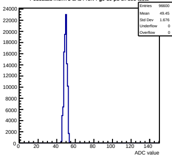
Pedestals mcm73-2A14-refv4-g0-s0-p1 ch 108 test1
