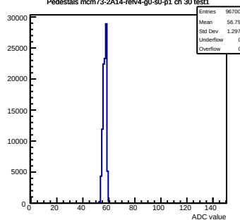
Pedestals mcm73-2A14-refv4-g0-s0-p1 ch 30 test1
