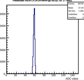
Pedestals mcm73-2A14-refv4-g0-s0-p1 ch 17 test1
