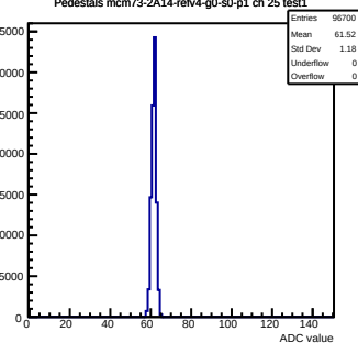
Pedestals mcm73-2A14-refv4-g0-s0-p1 ch 25 test1
