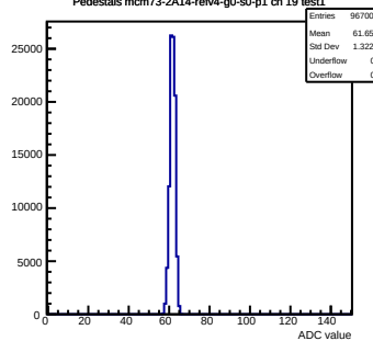
Pedestals mcm73-2A14-refv4-g0-s0-p1 ch 19 test1
