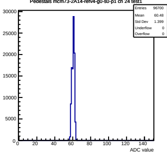
Pedestals mcm73-2A14-refv4-g0-s0-p1 ch 24 test1
