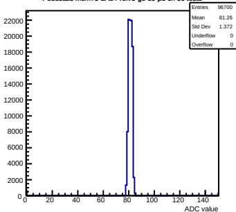
Pedestals mcm73-2A14-refv5-g0-s0-p1 ch 82 test1
