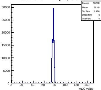
Pedestals mcm73-2A14-refv5-g0-s0-p1 ch 94 test1
