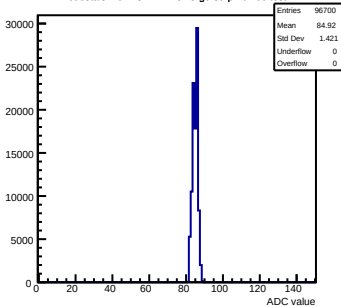
Pedestals mcm73-2A14-refv5-g0-s0-p1 ch 86 test1
