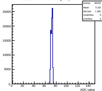
Pedestals mcm73-2A14-refv5-g0-s0-p1 ch 93 test1
