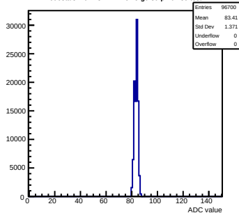
Pedestals mcm73-2A14-refv5-g0-s0-p1 ch 85 test1
