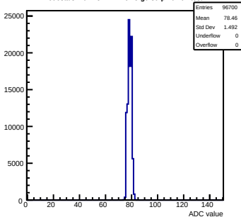
Pedestals mcm73-2A14-refv5-g0-s0-p1 ch 92 test1
