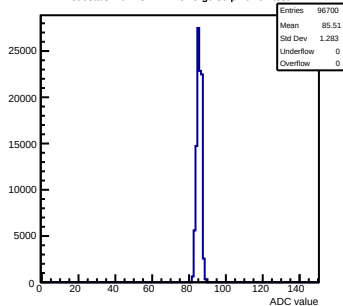
Pedestals mcm73-2A14-refv5-g0-s0-p1 ch 87 test1
