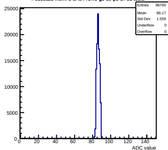
Pedestals mcm73-2A14-refv5-g0-s0-p1 ch 81 test1
