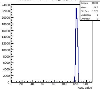
Pedestals mcm73-2A14- rev6 -g0-s0-p1 ch 84 test1
