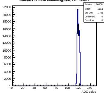
Pedestals mcm73-2A14-refv6-g0-s0-p1 ch 10 test1
