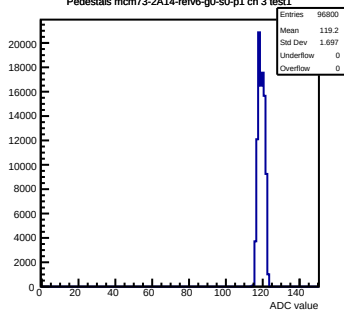
Pedestals mcm73-2A14-refv6-g0-s0-p1 ch 3 test1
