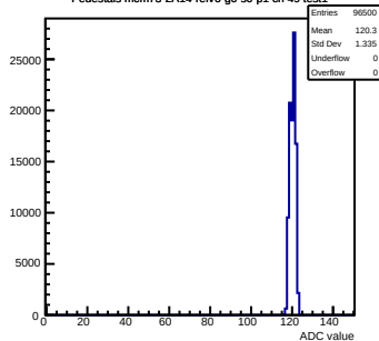
Pedestals mcm73-2A14-refv6-g0-s0-p1 ch 49 test1
