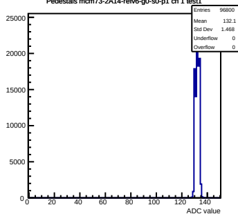
Pedestals mcm73-2A14-refv6-g0-s0-p1 ch 1 test1
