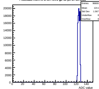
Pedestals mcm73-2A14-refv6-g0-s0-p1 ch 66 test1
