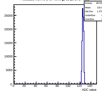
Pedestals mcm73-2A14- rev6 -g0-s0-p1 ch 87 test1
