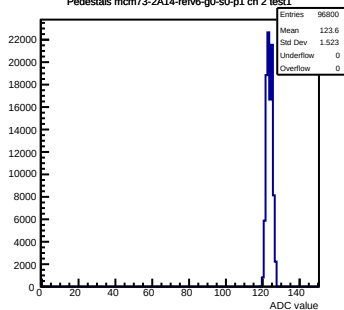
Pedestals mcm73-2A14-refv6-g0-s0-p1 ch 2 test1
