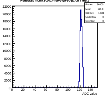
Pedestals mcm73-2A14-refv6-g0-s0-p1 ch 7 test1
