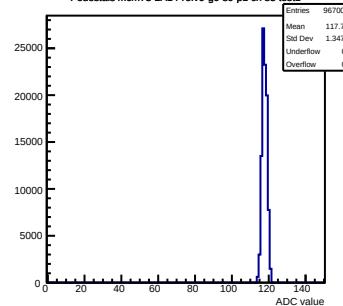
Pedestals mcm73-2A14- rev6 -g0-s0-p1 ch 83 test1
