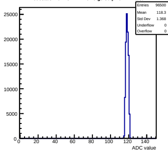
Pedestals mcm73-2A14-relv6-g0-s0-p1 ch 121 test1
