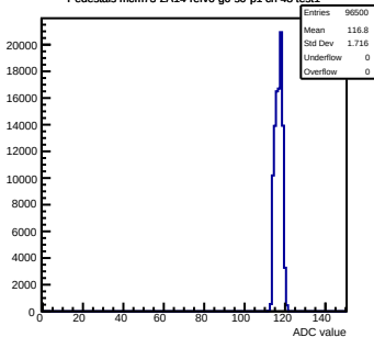
Pedestals mcm73-2A14-refv6-g0-s0-p1 ch 48 test1
