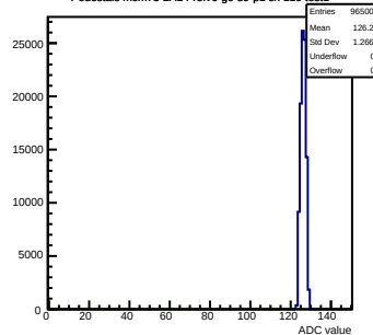
Pedestals mcm73-2A14-relv6-g0-s0-p1 ch 119 test1
