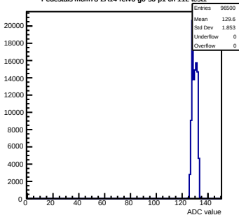
Pedestals mcm73-2A14-relv6-g0-s0-p1 ch 112 test1
