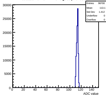
Pedestals mcm73-2A14- rev6 -g0-s0-p1 ch 93 test1
