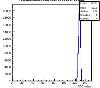
Pedestals mcm80-1016-refV0-g0-s0-p1 ch 83 test1
