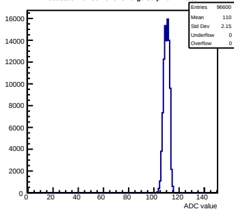
Pedestals mcm80-1016-refV0-g0-s0-p1 ch 42 test1
