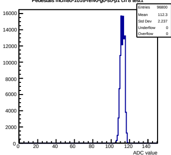
Pedestals mcm80-1016-refv0-g0-s0-p1 ch 8 test1
