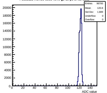
Pedestals mcm80-1016-refV0-g0-s0-p1 ch 89 test1
