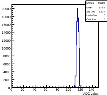
Pedestals mcm80-1016-refV0-g0-s0-p1 ch 61 test1
