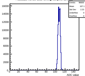
Pedestals mcm80-1016-refV0-g0-s0-p1 ch 38 test1
