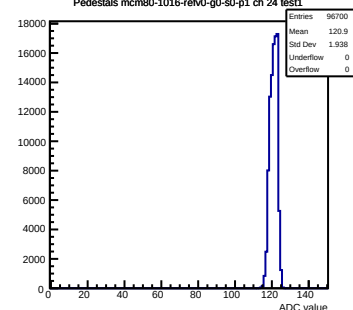
Pedestals mcm80-1016-refV0-g0-s0-p1 ch 24 test1
