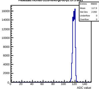
Pedestals mcm80-1016-refv0-g0-s0-p1 ch 5 test1
