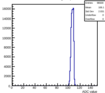
Pedestals mcm80-1016-refV0-g0-s0-p1 ch 62 test1
