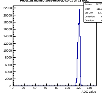
Pedestals mcm80-1016-refV0-g0-s0-p1 ch 23 test1
