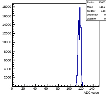
Pedestals mcm80-1016-refV0-g0-s0-p1 ch 111 test1
