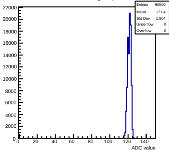
Pedestals mcm80-1016-refV0-g0-s0-p1 ch 60 test1
