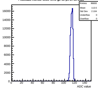
Pedestals mcm80-1016-refV0-g0-s0-p1 ch 66 test1
