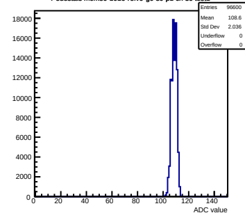
Pedestals mcm80-1016-refV0-g0-s0-p1 ch 36 test1
