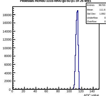
Pedestals mcm80-1016-refV0-g0-s0-p1 ch 26 test1
