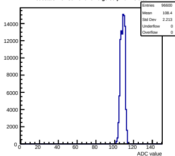
Pedestals mcm80-1016-refV0-g0-s0-p1 ch 43 test1
