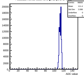
Pedestals mcm80-1016-refV0-g0-s0-p1 ch 37 test1
