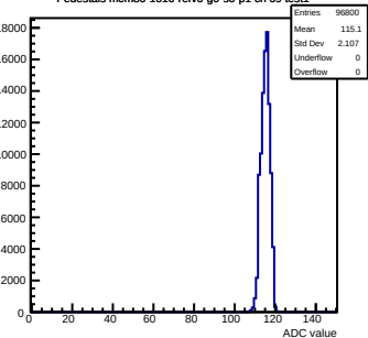
Pedestals mcm80-1016-refV0-g0-s0-p1 ch 69 test1
