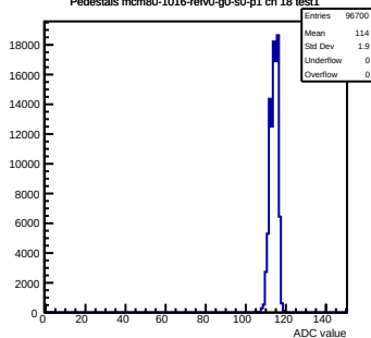
Pedestals mcm80-1016-refV0-g0-s0-p1 ch 18 test1
