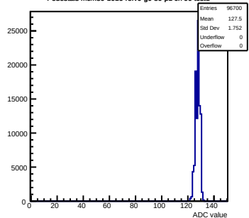
Pedestals mcm80-1016-refV0-g0-s0-p1 ch 90 test1
