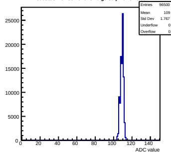
Pedestals mcm80-1016-refV0-g0-s0-p1 ch 51 test1
