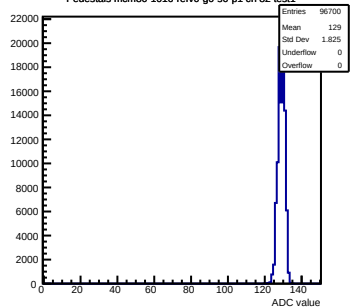
Pedestals mcm80-1016-refV0-g0-s0-p1 ch 82 test1
