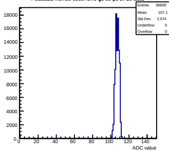
Pedestals mcm80-1016-refV0-g0-s0-p1 ch 39 test1
