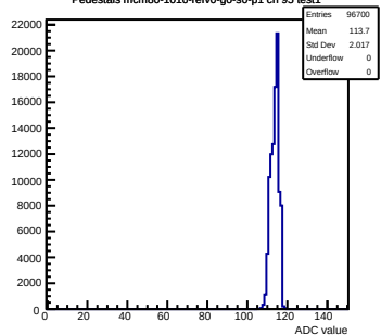
Pedestals mcm80-1016-refV0-g0-s0-p1 ch 95 test1
