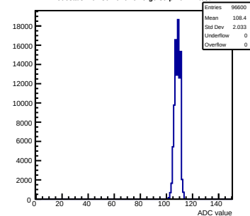
Pedestals mcm80-1016-refV0-g0-s0-p1 ch 44 test1
