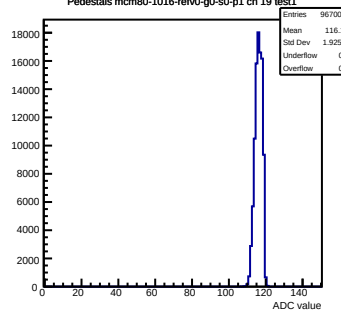
Pedestals mcm80-1016-refV0-g0-s0-p1 ch 19 test1
