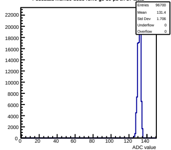
Pedestals mcm80-1016-refV0-g0-s0-p1 ch 87 test1
