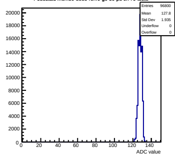
Pedestals mcm80-1016-refV0-g0-s0-p1 ch 79 test1
