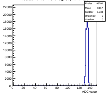
Pedestals mcm80-1016-refV0-g0-s0-p1 ch 91 test1
