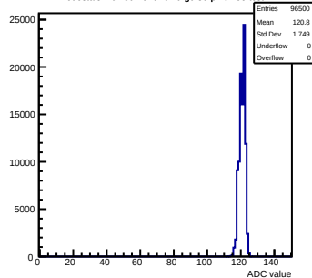
Pedestals mcm80-1016-refV0-g0-s0-p1 ch 55 test1
