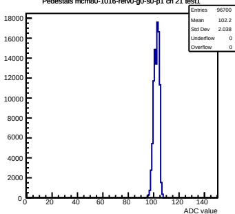
Pedestals mcm80-1016-refV0-g0-s0-p1 ch 21 test1
