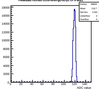
Pedestals mcm80-1016-refv0-g0-s0-p1 ch 9 test1
