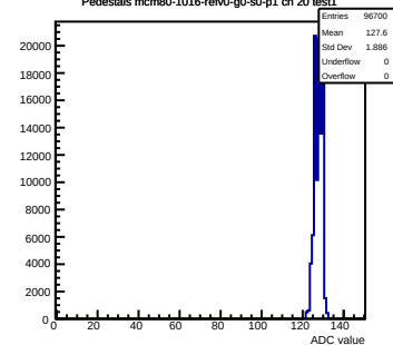
Pedestals mcm80-1016-refV0-g0-s0-p1 ch 20 test1
