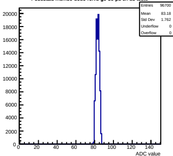
Pedestals mcm80-1016-refv1-g0-s0-p1 ch 18 test1
