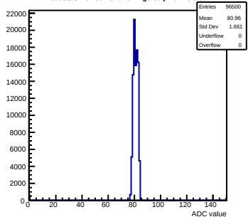
Pedestals mcm80-1016-refv1-g0-s0-p1 ch 49 test1
