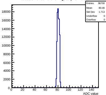
Pedestals mcm80-1016-refv1-g0-s0-p1 ch 26 test1
