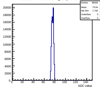
Pedestals mcm80-1016-refv1-g0-s0-p1 ch 50 test1
