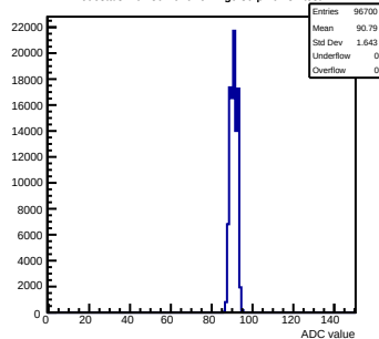
Pedestals mcm80-1016-refv1-g0-s0-p1 ch 31 test1
