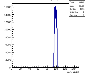
Pedestals mcm80-1016-refv1-g0-s0-p1 ch 48 test1
