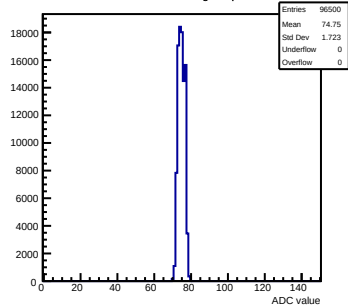
Pedestals mcm80-1016-refv1-g0-s0-p1 ch 62 test1
