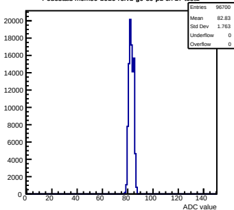
Pedestals mcm80-1016-refv1-g0-s0-p1 ch 17 test1
