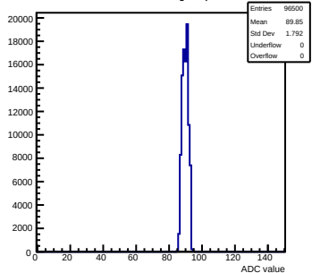
Pedestals mcm80-1016-refv1-g0-s0-p1 ch 57 test1
