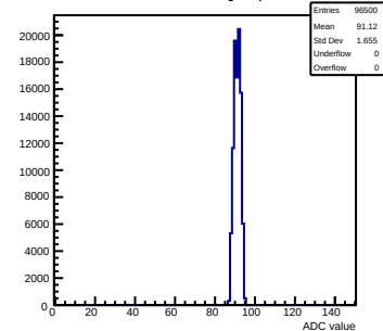
Pedestals mcm80-1016-refv1-g0-s0-p1 ch 60 test1
