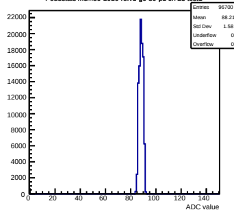
Pedestals mcm80-1016-refv1-g0-s0-p1 ch 23 test1
