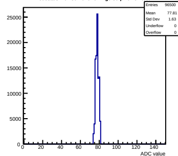
Pedestals mcm80-1016-refv1-g0-s0-p1 ch 51 test1
