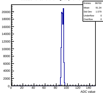
Pedestals mcm80-1016-refv1-g0-s0-p1 ch 25 test1
