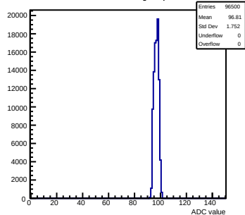
Pedestals mcm80-1016-refv1-g0-s0-p1 ch 58 test1
