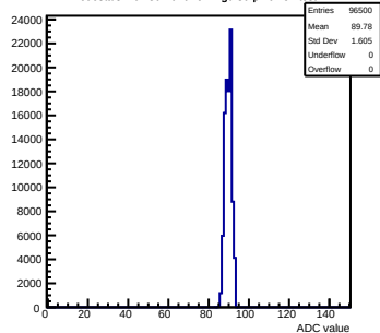
Pedestals mcm80-1016-refv1-g0-s0-p1 ch 54 test1
