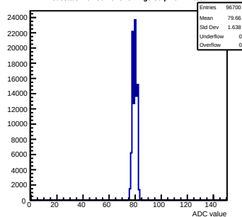
Pedestals mcm80-1016-refv1-g0-s0-p1 ch 27 test1
