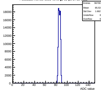
Pedestals mcm80-1016-refv1-g0-s0-p1 ch 19 test1
