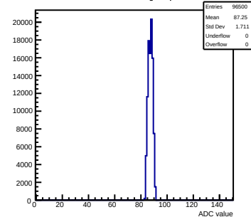
Pedestals mcm80-1016-refv1-g0-s0-p1 ch 56 test1
