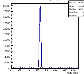
Pedestals mcm80-1016-refv2-g0-s0-p1 ch 19 test1
