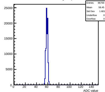
Pedestals mcm80-1016-refv2-g0-s0-p1 ch 27 test1
