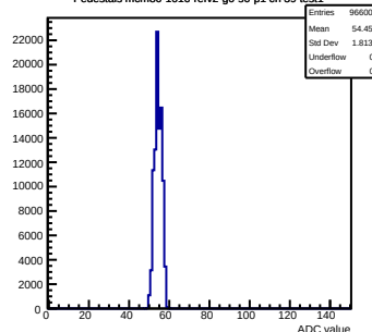
Pedestals mcm80-1016-refv2-g0-s0-p1 ch 39 test1
