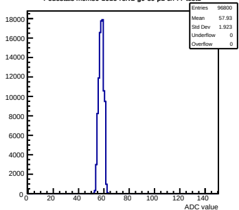
Pedestals mcm80-1016-refv2-g0-s0-p1 ch 77 test1
