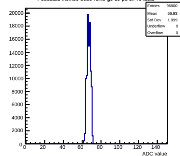
Pedestals mcm80-1016-refv2-g0-s0-p1 ch 76 test1
