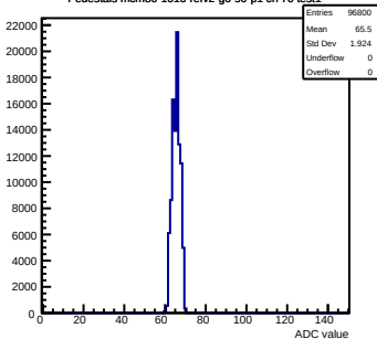
Pedestals mcm80-1016-refv2-g0-s0-p1 ch 70 test1
