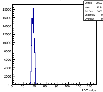
Pedestals mcm80-1016-refv3-g0-s0-p1 ch 110 test1
