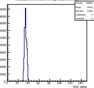
Pedestals mcm80-1016-refv3-g0-s0-p1 ch 5 test1
