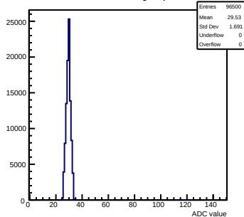
Pedestals mcm80-1016-refv3-g0-s0-p1 ch 61 test1
