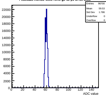
Pedestals mcm80-1016-refv3-g0-s0-p1 ch 81 test1
