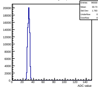
Pedestals mcm80-1016-refv3-g0-s0-p1 ch 55 test1
