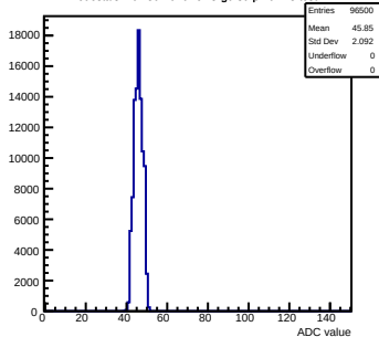
Pedestals mcm80-1016-refv3-g0-s0-p1 ch 48 test1
