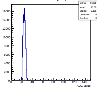
Pedestals mcm80-1016-refv3-g0-s0-p1 ch 11 test1
