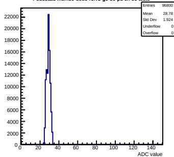
Pedestals mcm80-1016-refv3-g0-s0-p1 ch 66 test1
