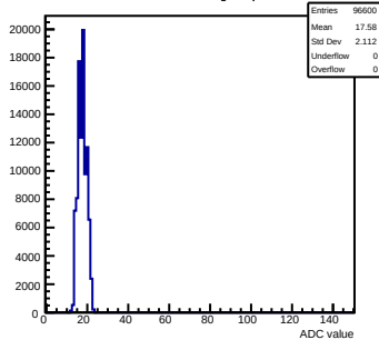
Pedestals mcm80-1016-refv3-g0-s0-p1 ch 102 test1
