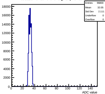
Pedestals mcm80-1016-refv3-g0-s0-p1 ch 68 test1
