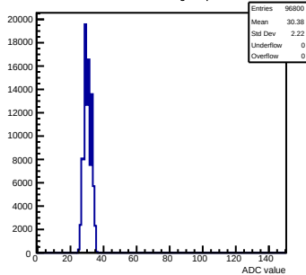
Pedestals mcm80-1016-refv3-g0-s0-p1 ch 74 test1
