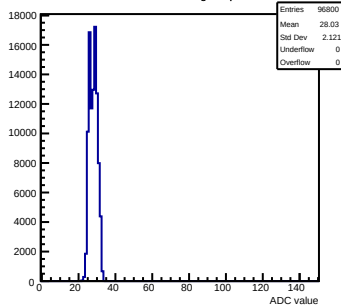
Pedestals mcm80-1016-refv3-g0-s0-p1 ch 78 test1
