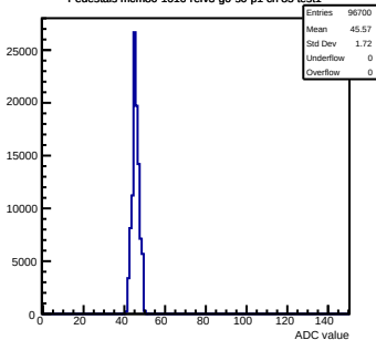
Pedestals mcm80-1016-refv3-g0-s0-p1 ch 85 test1
