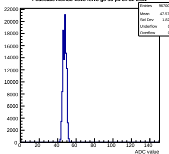
Pedestals mcm80-1016-refv3-g0-s0-p1 ch 82 test1
