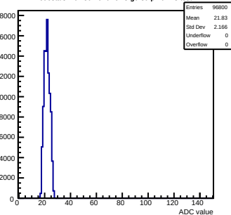
Pedestals mcm80-1016-refv3-g0-s0-p1 ch 13 test1
