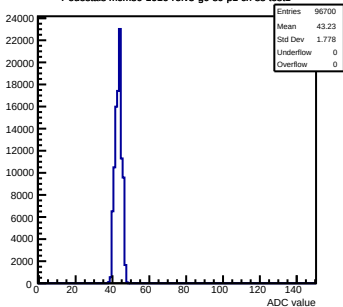
Pedestals mcm80-1016-refv3-g0-s0-p1 ch 88 test1
