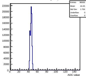
Pedestals mcm80-1016-refv3-g0-s0-p1 ch 54 test1
