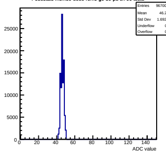
Pedestals mcm80-1016-refv3-g0-s0-p1 ch 90 test1
