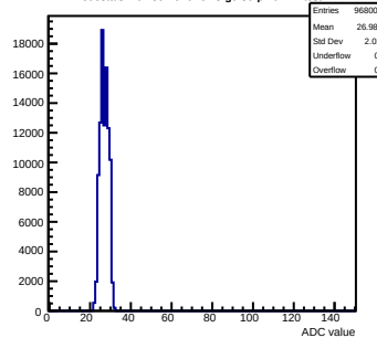
Pedestals mcm80-1016-refv3-g0-s0-p1 ch 71 test1
