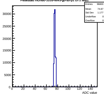
Pedestals mcm80-1016-rev5-g0-s0-p1 ch 2 test1
