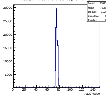
Pedestals mcm80-1016-refV5-g0-s0-p1 ch 102 test1
