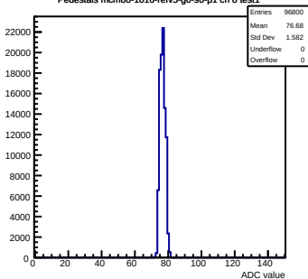
Pedestals mcm80-1016-rev5-g0-s0-p1 ch 8 test1
