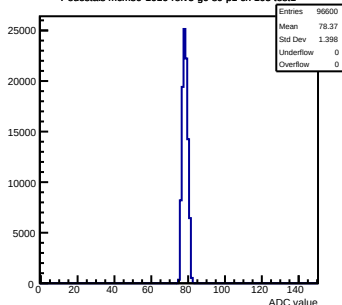
Pedestals mcm80-1016-refV5-g0-s0-p1 ch 105 test1
