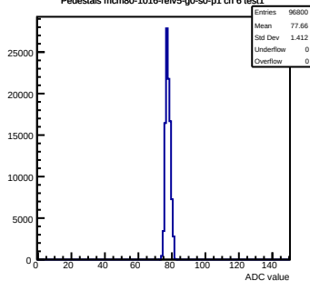
Pedestals mcm80-1016-rev5-g0-s0-p1 ch 6 test1
