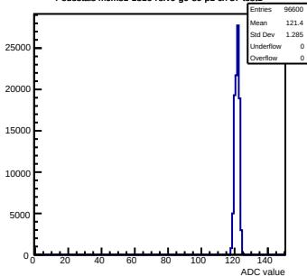
Pedestals mcm81-1816-refV0-g0-s0-p1 ch 37 test1
