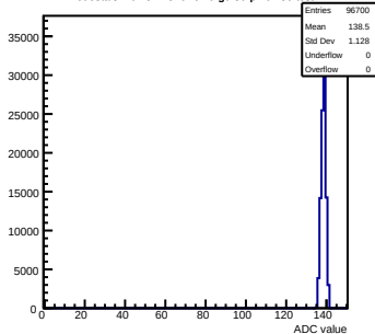
Pedestals mcm81-1816-refV0-g0-s0-p1 ch 86 test1
