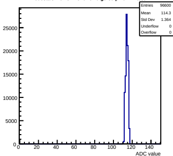
Pedestals mcm81-1816-refV0-g0-s0-p1 ch 41 test1
