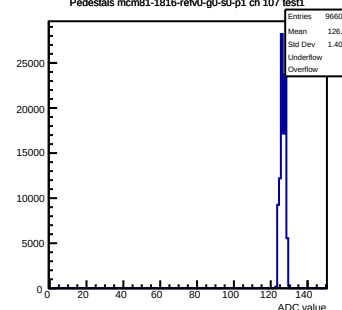
Pedestals mcm81-1816-refV0-g0-s0-p1 ch 107 test1
