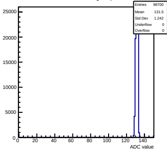
Pedestals mcm81-1816-refV0-g0-s0-p1 ch 88 test1
