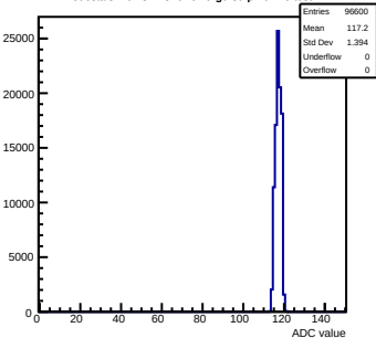
Pedestals mcm81-1816-refV0-g0-s0-p1 ch 40 test1
