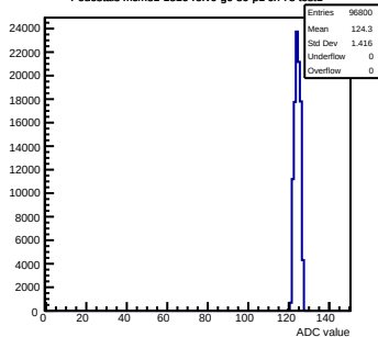
Pedestals mcm81-1816-refV0-g0-s0-p1 ch 78 test1
