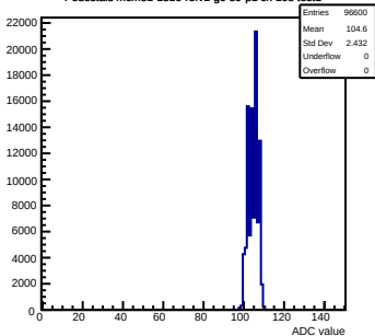
Pedestals mcm81-1816-refv1-g0-s0-p1 ch 104 test1
