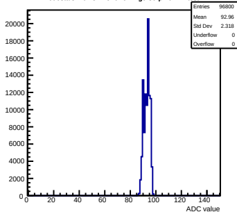
Pedestals mcm81-1816-refv1-g0-s0-p1 ch 71 test1
