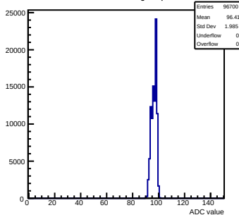
Pedestals mcm81-1816-refv1-g0-s0-p1 ch 25 test1
