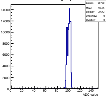
Pedestals mcm81-1816-refv1-g0-s0-p1 ch 16 test1
