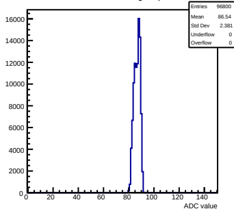
Pedestals mcm81-1816-refv1-g0-s0-p1 ch 9 test1
