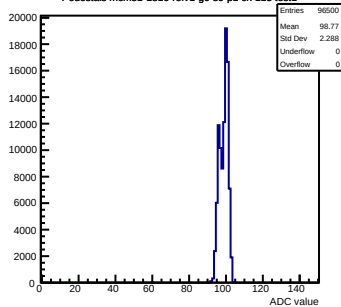
Pedestals mcm81-1816-refv1-g0-s0-p1 ch 113 test1
