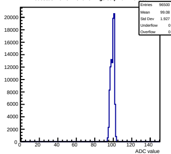
Pedestals mcm81-1816-refv1-g0-s0-p1 ch 119 test1
