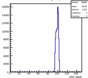
Pedestals mcm81-1816-refv1-g0-s0-p1 ch 67 test1
