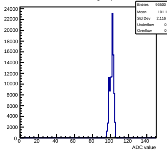
Pedestals mcm81-1816-refv1-g0-s0-p1 ch 123 test1
