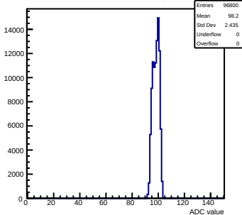
Pedestals mcm81-1816-refv1-g0-s0-p1 ch 4 test1
