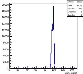
Pedestals mcm81-1816-refv1-g0-s0-p1 ch 1 test1
