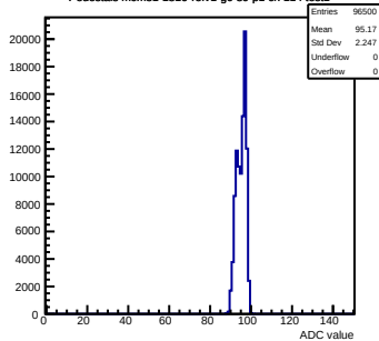
Pedestals mcm81-1816-refv1-g0-s0-p1 ch 114 test1
