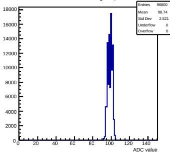
Pedestals mcm81-1816-refv1-g0-s0-p1 ch 8 test1
