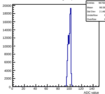
Pedestals mcm81-1816-refv1-g0-s0-p1 ch 27 test1
