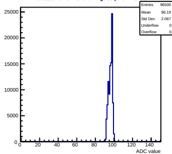
Pedestals mcm81-1816-refv1-g0-s0-p1 ch 118 test1
