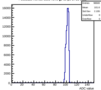
Pedestals mcm81-1816-refv1-g0-s0-p1 ch 53 test1
