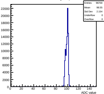
Pedestals mcm81-1816-refv1-g0-s0-p1 ch 28 test1
