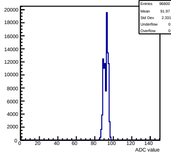
Pedestals mcm81-1816-refv1-g0-s0-p1 ch 6 test1
