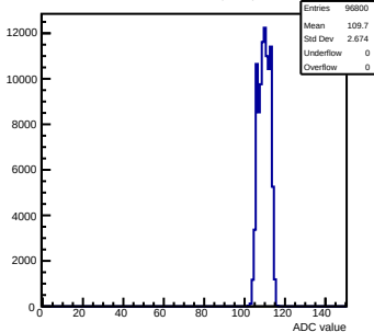
Pedestals mcm81-1816-refv1-g0-s0-p1 ch 0 test1
