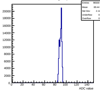
Pedestals mcm81-1816-refv1-g0-s0-p1 ch 122 test1
