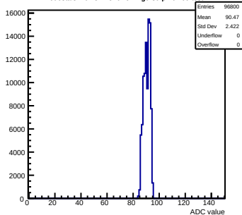
Pedestals mcm81-1816-refv1-g0-s0-p1 ch 69 test1
