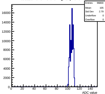
Pedestals mcm81-1816-refv1-g0-s0-p1 ch 64 test1
