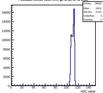
Pedestals mcm81-1816-refv1-g0-s0-p1 ch 48 test1
