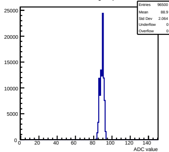
Pedestals mcm81-1816-refv1-g0-s0-p1 ch 126 test1
