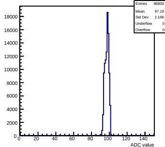
Pedestals mcm81-1816-refv1-g0-s0-p1 ch 2 test1
