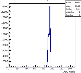
Pedestals mcm81-1816-refv1-g0-s0-p1 ch 60 test1
