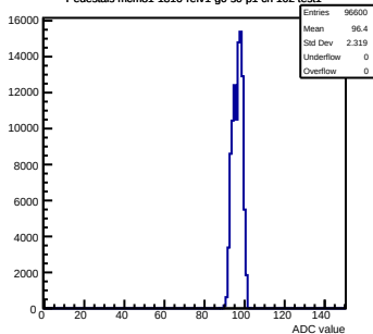
Pedestals mcm81-1816-refv1-g0-s0-p1 ch 102 test1
