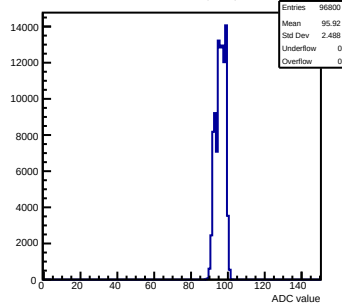
Pedestals mcm81-1816-refv1-g0-s0-p1 ch 3 test1
