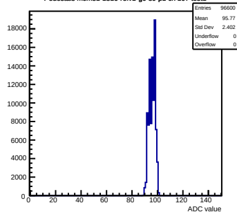
Pedestals mcm81-1816-refv1-g0-s0-p1 ch 107 test1
