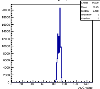
Pedestals mcm81-1816-refv1-g0-s0-p1 ch 68 test1
