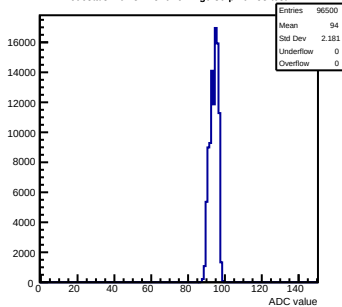
Pedestals mcm81-1816-refv1-g0-s0-p1 ch 58 test1
