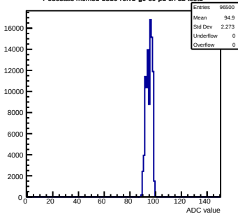
Pedestals mcm81-1816-refv1-g0-s0-p1 ch 52 test1
