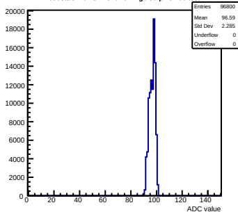
Pedestals mcm81-1816-refv1-g0-s0-p1 ch 66 test1
