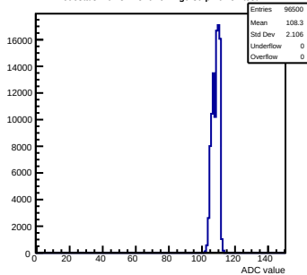
Pedestals mcm81-1816-refv1-g0-s0-p1 ch 57 test1
