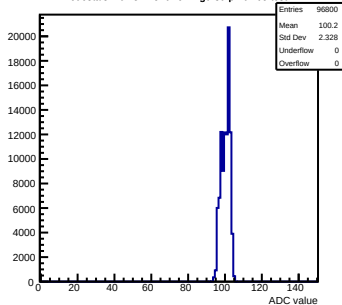
Pedestals mcm81-1816-refv1-g0-s0-p1 ch 65 test1
