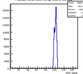
Pedestals mcm81-1816-refv1-g0-s0-p1 ch 99 test1
