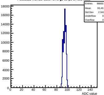
Pedestals mcm81-1816-refv1-g0-s0-p1 ch 109 test1
