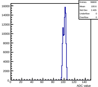
Pedestals mcm81-1816-refv1-g0-s0-p1 ch 12 test1
