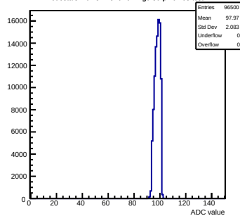
Pedestals mcm81-1816-refv1-g0-s0-p1 ch 63 test1
