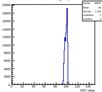
Pedestals mcm81-1816-refv1-g0-s0-p1 ch 61 test1
