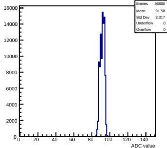
Pedestals mcm81-1816-refv1-g0-s0-p1 ch 13 test1
