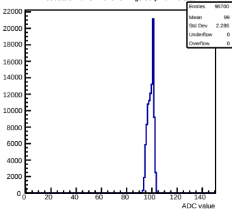
Pedestals mcm81-1816-refv1-g0-s0-p1 ch 18 test1
