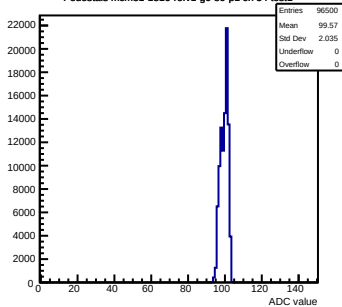
Pedestals mcm81-1816-refv1-g0-s0-p1 ch 54 test1
