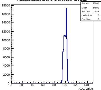
Pedestals mcm81-1816-refv1-g0-s0-p1 ch 96 test1
