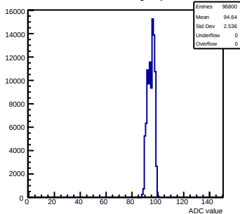
Pedestals mcm81-1816-refv1-g0-s0-p1 ch 74 test1
