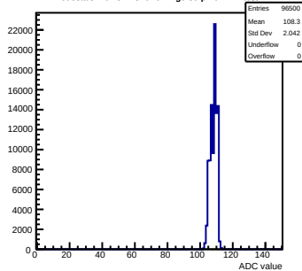
Pedestals mcm81-1816-refv1-g0-s0-p1 ch 117 test1
