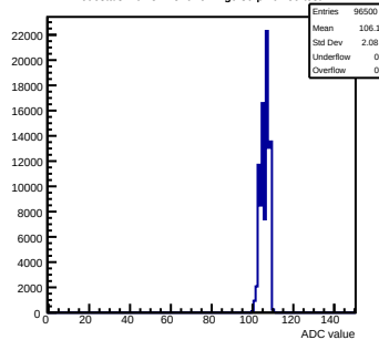
Pedestals mcm81-1816-refv1-g0-s0-p1 ch 59 test1
