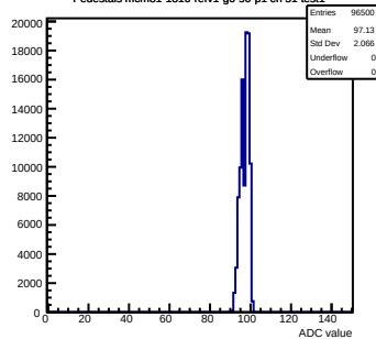
Pedestals mcm81-1816-refv1-g0-s0-p1 ch 51 test1
