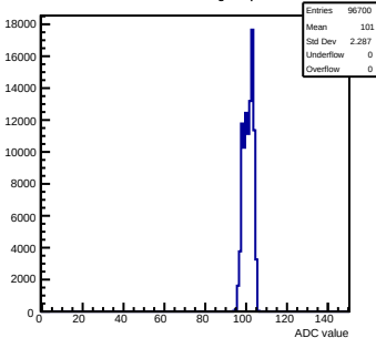
Pedestals mcm81-1816-refv1-g0-s0-p1 ch 30 test1
