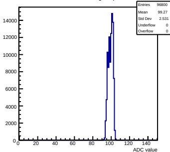
Pedestals mcm81-1816-refv1-g0-s0-p1 ch 72 test1
