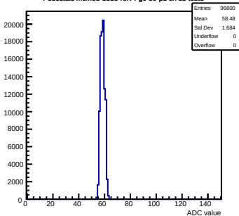
Pedestals mcm81-1816-rtv4-g0-s0-p1 ch 15 test1
