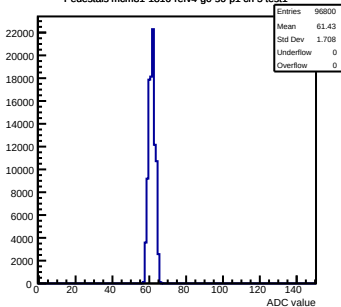
Pedestals mcm81-1816-rtv4-g0-s0-p1 ch 5 test1
