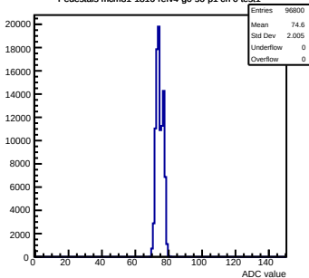
Pedestals mcm81-1816-rtv4-g0-s0-p1 ch 0 test1
