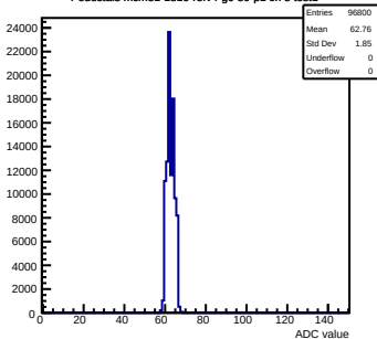
Pedestals mcm81-1816-rtv4-g0-s0-p1 ch 8 test1
