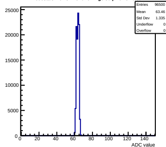
Pedestals mcm81-1816-refv4-g0-s0-p1 ch 54 test1
