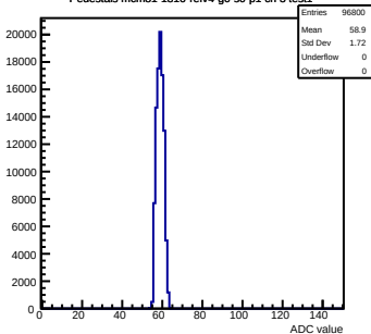
Pedestals mcm81-1816-rtv4-g0-s0-p1 ch 3 test1
