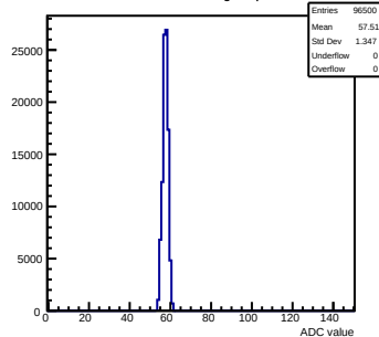
Pedestals mcm81-1816-refv4-g0-s0-p1 ch 58 test1
