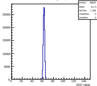
Pedestals mcm81-1816-refv4-g0-s0-p1 ch 61 test1
