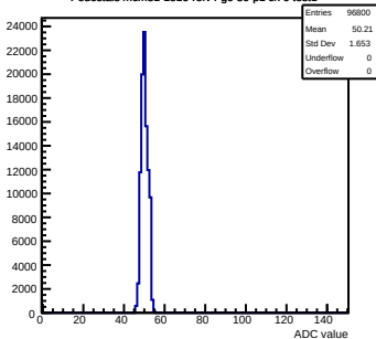
Pedestals mcm81-1816-rtv4-g0-s0-p1 ch 9 test1
