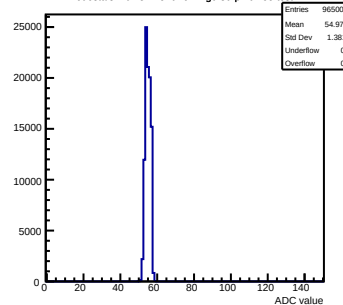
Pedestals mcm81-1816-refv4-g0-s0-p1 ch 55 test1
