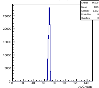
Pedestals mcm81-1816-refv4-g0-s0-p1 ch 62 test1
