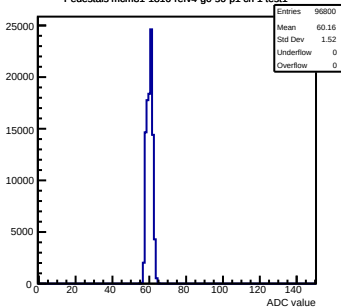
Pedestals mcm81-1816-rtv4-g0-s0-p1 ch 1 test1
