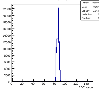
Pedestals mcm81-1816-refV5-g0-s0-p1 ch 109 test1
