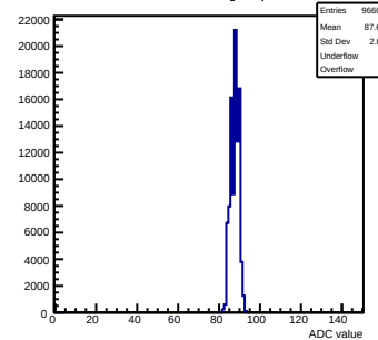
Pedestals mcm81-1816-refV5-g0-s0-p1 ch 107 test1
