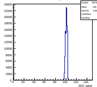
Pedestals mcm81-1816-refV5-g0-s0-p1 ch 95 test1
