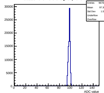
Pedestals mcm81-1816-refV5-g0-s0-p1 ch 87 test1
