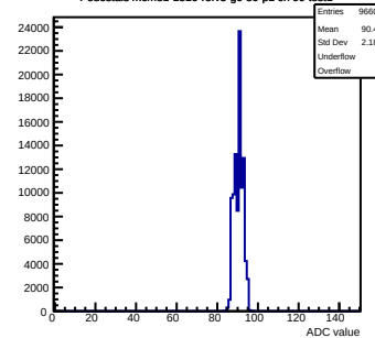
Pedestals mcm81-1816-refV5-g0-s0-p1 ch 99 test1
