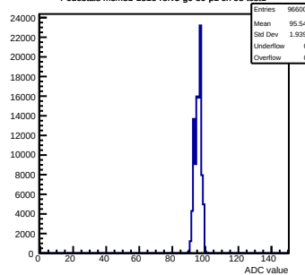
Pedestals mcm81-1816-refV5-g0-s0-p1 ch 98 test1
