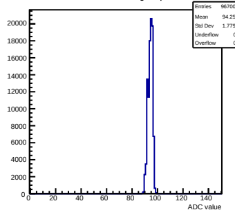
Pedestals mcm81-1816-refV5-g0-s0-p1 ch 90 test1
