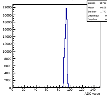
Pedestals mcm81-1816-refV5-g0-s0-p1 ch 89 test1
