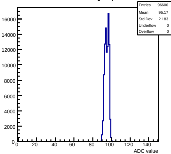
Pedestals mcm81-1816-refV5-g0-s0-p1 ch 100 test1
