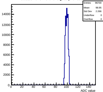
Pedestals mcm81-1816-refV5-g0-s0-p1 ch 80 test1
