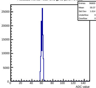
Pedestals mcm82-7015-refv2-g0-s0-p1 ch 75 test1
