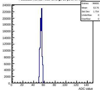
Pedestals mcm82-7015-refv2-g0-s0-p1 ch 14 test1
