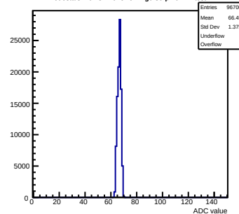
Pedestals mcm82-7015-refv2-g0-s0-p1 ch 27 test1
