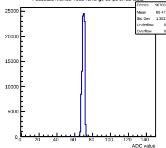
Pedestals mcm82-7015-refv2-g0-s0-p1 ch 22 test1
