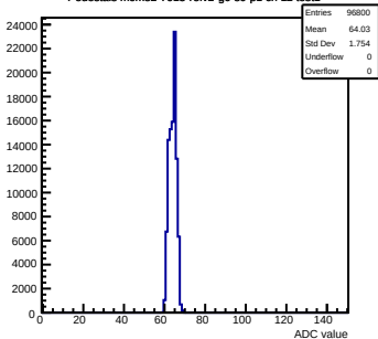
Pedestals mcm82-7015-refv2-g0-s0-p1 ch 12 test1
