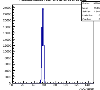
Pedestals mcm82-7015-refv2-g0-s0-p1 ch 18 test1
