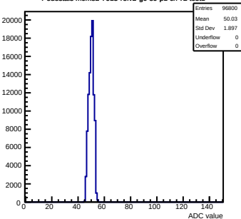
Pedestals mcm82-7015-refv2-g0-s0-p1 ch 72 test1
