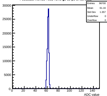
Pedestals mcm82-7015-refv2-g0-s0-p1 ch 21 test1
