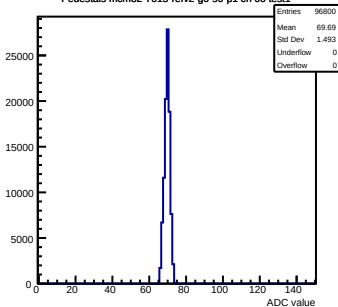
Pedestals mcm82-7015-refv2-g0-s0-p1 ch 66 test1
