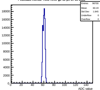
Pedestals mcm82-7015-refv2-g0-s0-p1 ch 16 test1
