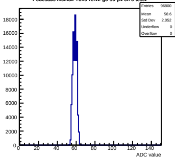
Pedestals mcm82-7015-refv2-g0-s0-p1 ch 0 test1
