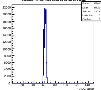
Pedestals mcm82-7015-refv2-g0-s0-p1 ch 6 test1
