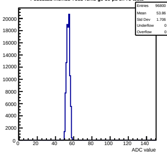
Pedestals mcm82-7015-refv2-g0-s0-p1 ch 79 test1
