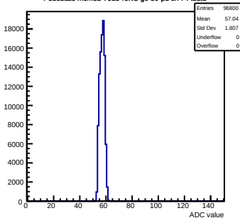
Pedestals mcm82-7015-refv2-g0-s0-p1 ch 74 test1
