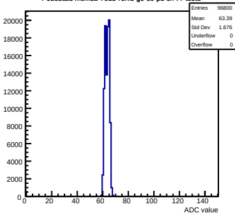
Pedestals mcm82-7015-refv2-g0-s0-p1 ch 77 test1
