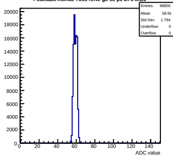
Pedestals mcm82-7015-refv2-g0-s0-p1 ch 5 test1
