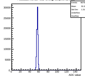
Pedestals mcm82-7015-refv2-g0-s0-p1 ch 23 test1
