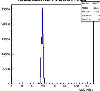
Pedestals mcm82-7015-refv2-g0-s0-p1 ch 71 test1
