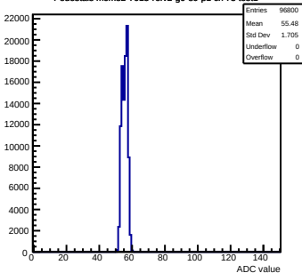
Pedestals mcm82-7015-refv2-g0-s0-p1 ch 73 test1
