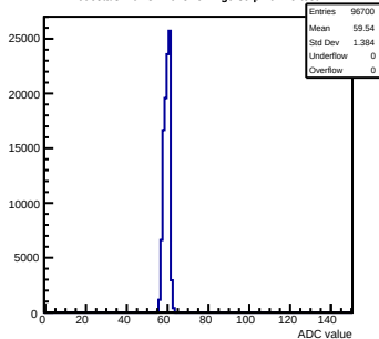
Pedestals mcm82-7015-refv2-g0-s0-p1 ch 29 test1
