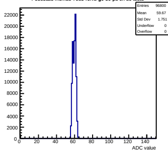
Pedestals mcm82-7015-refv2-g0-s0-p1 ch 10 test1
