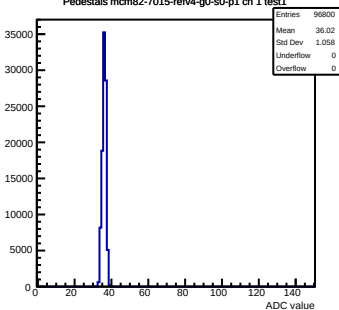
Pedestals mcm82-7015-refv4-g0-s0-p1 ch 1 test1
