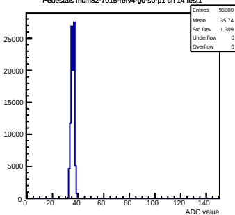
Pedestals mcm82-7015-refv4-g0-s0-p1 ch 14 test1
