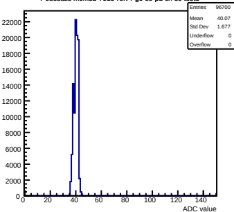
Pedestals mcm82-7015-refv4-g0-s0-p1 ch 80 test1
