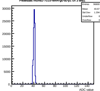
Pedestals mcm82-7015-refv4-g0-s0-p1 ch 3 test1
