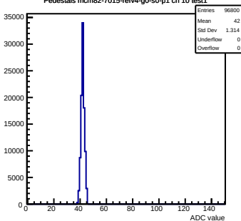
Pedestals mcm82-7015-refv4-g0-s0-p1 ch 10 test1
