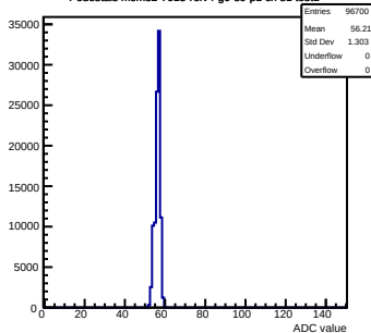
Pedestals mcm82-7015-refv4-g0-s0-p1 ch 81 test1
