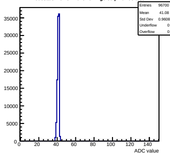
Pedestals mcm82-7015-refv4-g0-s0-p1 ch 93 test1
