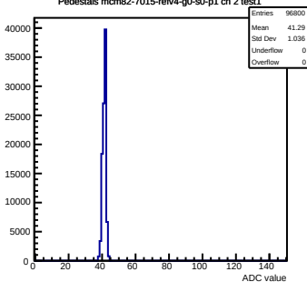
Pedestals mcm82-7015-refv4-g0-s0-p1 ch 2 test1
