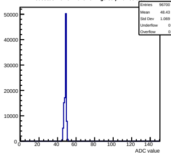
Pedestals mcm82-7015-refv4-g0-s0-p1 ch 85 test1
