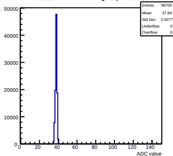
Pedestals mcm82-7015-refv4-g0-s0-p1 ch 89 test1
