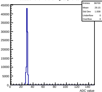
Pedestals mcm82-7015-refv4-g0-s0-p1 ch 88 test1
