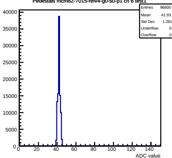
Pedestals mcm82-7015-refv4-g0-s0-p1 ch 6 test1
