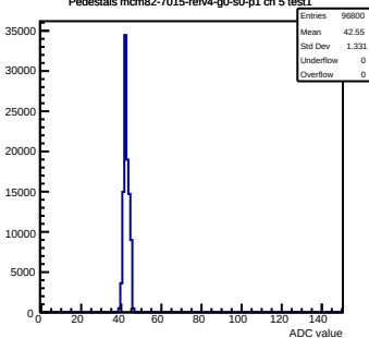
Pedestals mcm82-7015-refv4-g0-s0-p1 ch 5 test1
