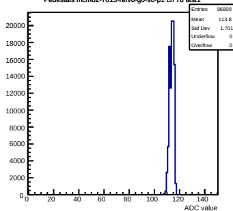
Pedestals mcm82-7015-refv6-g0-s0-p1 ch 78 test1
