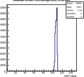
Pedestals mcm82-7015-refv6-g0-s0-p1 ch 69 test1
