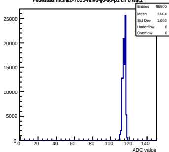
Pedestals mcm82-7015-relv6-g0-s0-p1 ch 6 test1
