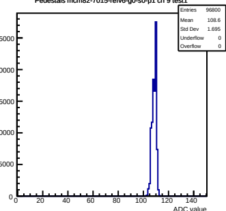
Pedestals mcm82-7015-relv6-g0-s0-p1 ch 9 test1
