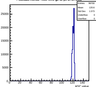
Pedestals mcm82-7015-refv6-g0-s0-p1 ch 84 test1
