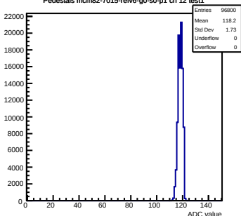
Pedestals mcm82-7015-relv6-g0-s0-p1 ch 12 test1
