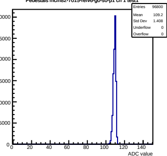
Pedestals mcm82-7015-relv6-g0-s0-p1 ch 1 test1
