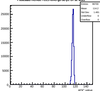
Pedestals mcm82-7015-refv6-g0-s0-p1 ch 92 test1
