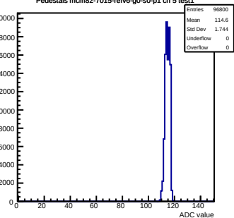
Pedestals mcm82-7015-relv6-g0-s0-p1 ch 5 test1
