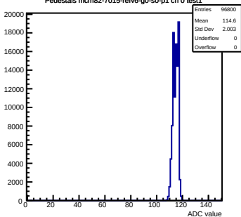
Pedestals mcm82-7015-relv6-g0-s0-p1 ch 0 test1
