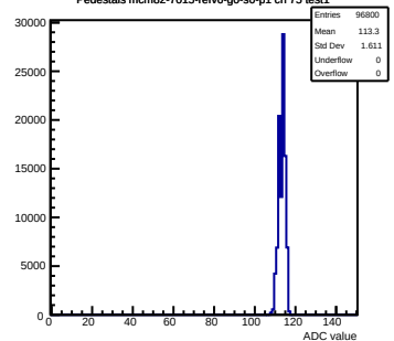
Pedestals mcm82-7015-refv6-g0-s0-p1 ch 75 test1
