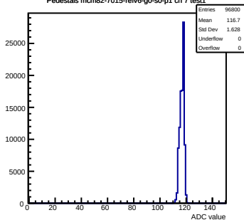
Pedestals mcm82-7015-relv6-g0-s0-p1 ch 7 test1
