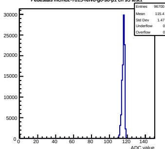
Pedestals mcm82-7015-refv6-g0-s0-p1 ch 95 test1
