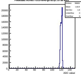
Pedestals mcm82-7015-refv6-g0-s0-p1 ch 68 test1
