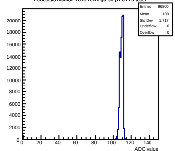
Pedestals mcm82-7015-refv6-g0-s0-p1 ch 79 test1
