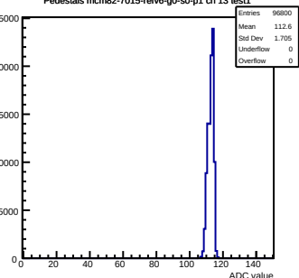
Pedestals mcm82-7015-relv6-g0-s0-p1 ch 13 test1
