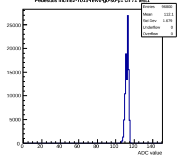
Pedestals mcm82-7015-refv6-g0-s0-p1 ch 71 test1
