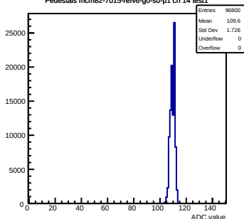
Pedestals mcm82-7015-relv6-g0-s0-p1 ch 14 test1
