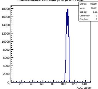
Pedestals mcm82-7015-refv6-g0-s0-p1 ch 72 test1
