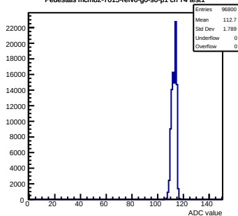
Pedestals mcm82-7015-refv6-g0-s0-p1 ch 74 test1
