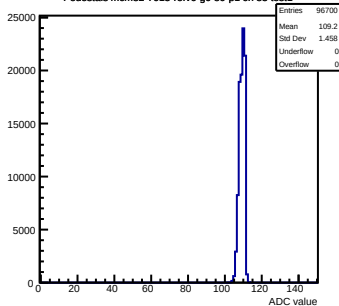
Pedestals mcm82-7015-refv6-g0-s0-p1 ch 83 test1
