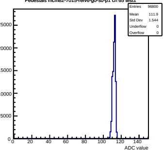
Pedestals mcm82-7015-refv6-g0-s0-p1 ch 65 test1
