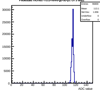
Pedestals mcm82-7015-relv6-g0-s0-p1 ch 3 test1
