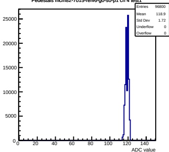
Pedestals mcm82-7015-relv6-g0-s0-p1 ch 4 test1
