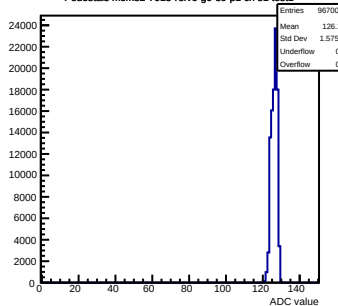
Pedestals mcm82-7015-refv6-g0-s0-p1 ch 81 test1
