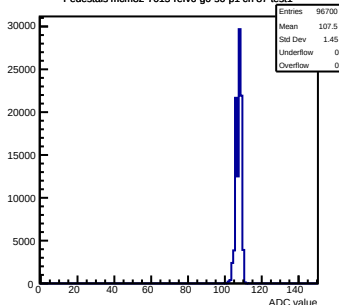
Pedestals mcm82-7015-refv6-g0-s0-p1 ch 87 test1
