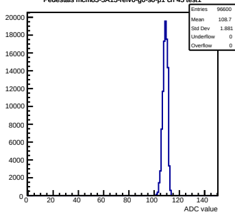
Pedestals mcm83-5A13-refV0-g0-s0-p1 ch 45 test1
