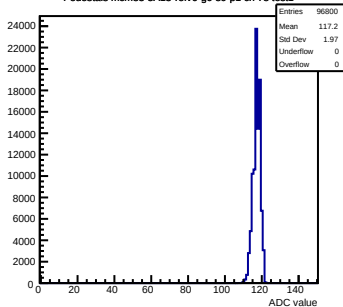
Pedestals mcm83-5A13-refV0-g0-s0-p1 ch 78 test1
