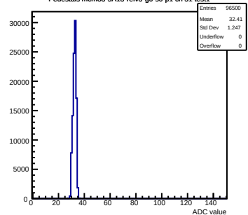
Pedestals mcm83-5A13-refv3-g0-s0-p1 ch 51 test1
