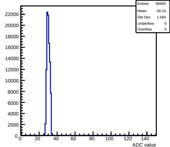
Pedestals mcm83-5A13-refv3-g0-s0-p1 ch 107 test1
