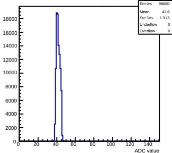
Pedestals mcm83-5A13-refv3-g0-s0-p1 ch 96 test1
