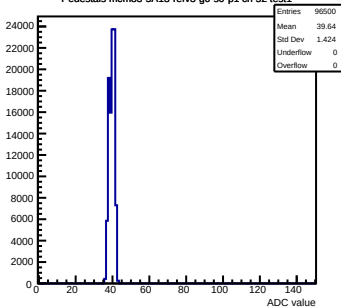
Pedestals mcm83-5A13-refv3-g0-s0-p1 ch 52 test1
