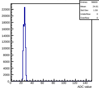
Pedestals mcm83-5A13-refv3-g0-s0-p1 ch 100 test1
