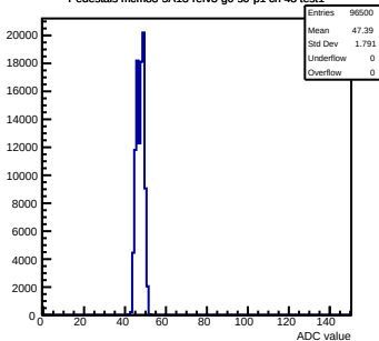
Pedestals mcm83-5A13-refv3-g0-s0-p1 ch 48 test1
