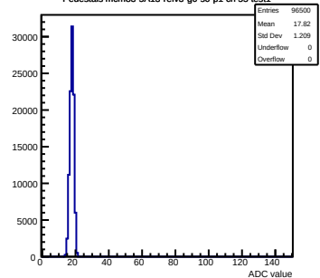
Pedestals mcm83-5A13-refv3-g0-s0-p1 ch 55 test1
