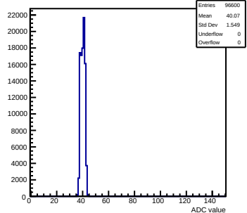
Pedestals mcm83-5A13-refv3-g0-s0-p1 ch 105 test1
