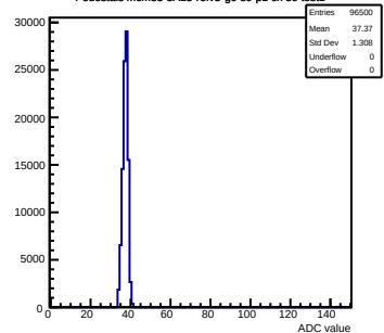
Pedestals mcm83-5A13-refv3-g0-s0-p1 ch 59 test1
