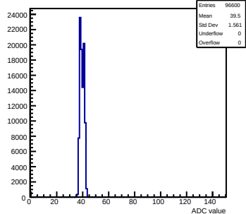
Pedestals mcm83-5A13-refv3-g0-s0-p1 ch 111 test1
