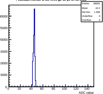
Pedestals mcm83-5A13-refv3-g0-s0-p1 ch 53 test1
