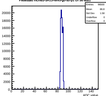
Pedestals mcm83-5A13-refV5-g0-s0-p1 ch 56 test1
