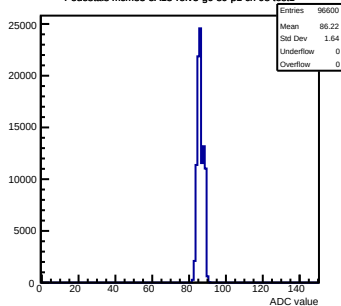
Pedestals mcm83-5A13-relv5-g0-s0-p1 ch 98 test1
