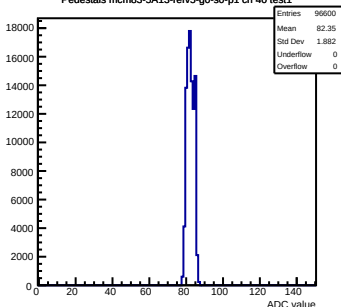
Pedestals mcm83-5A13-refv5-g0-s0-p1 ch 40 test1
