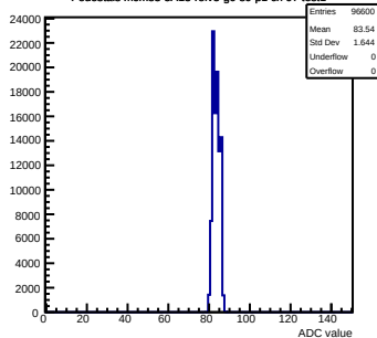
Pedestals mcm83-5A13-relv5-g0-s0-p1 ch 97 test1
