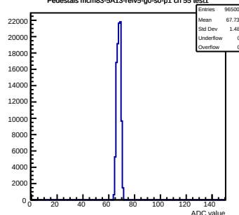
Pedestals mcm83-5A13-refV5-g0-s0-p1 ch 55 test1
