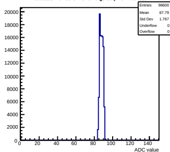
Pedestals mcm83-5A13-relv5-g0-s0-p1 ch 105 test1
