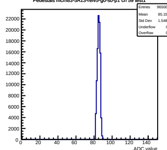
Pedestals mcm83-5A13-refV5-g0-s0-p1 ch 59 test1
