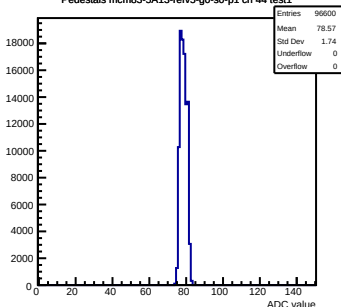
Pedestals mcm83-5A13-refv5-g0-s0-p1 ch 44 test1
