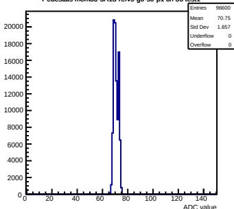
Pedestals mcm83-5A13-refv5-g0-s0-p1 ch 36 test1
