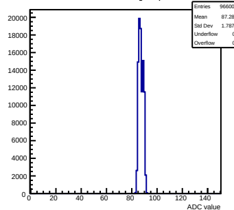
Pedestals mcm83-5A13-relv5-g0-s0-p1 ch 111 test1
