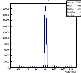
Pedestals mcm83-5A13-relv5-g0-s0-p1 ch 103 test1
