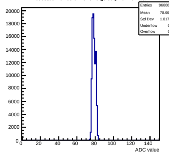
Pedestals mcm83-5A13-relv5-g0-s0-p1 ch 107 test1
