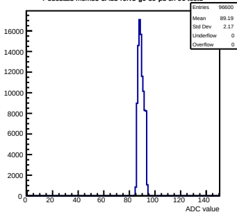
Pedestals mcm83-5A13-relv5-g0-s0-p1 ch 96 test1
