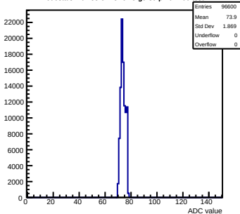
Pedestals mcm83-5A13-relv5-g0-s0-p1 ch 100 test1
