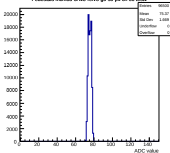
Pedestals mcm83-5A13-refV5-g0-s0-p1 ch 50 test1
