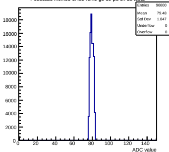
Pedestals mcm83-5A13-refv5-g0-s0-p1 ch 32 test1
