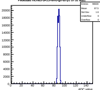
Pedestals mcm83-5A13-refV5-g0-s0-p1 ch 52 test1
