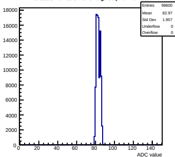
Pedestals mcm83-5A13-relv5-g0-s0-p1 ch 104 test1
