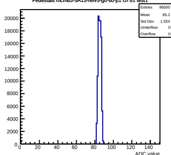
Pedestals mcm83-5A13-refV5-g0-s0-p1 ch 61 test1
