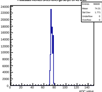
Pedestals mcm83-5A13-refv5-g0-s0-p1 ch 43 test1
