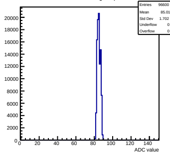
Pedestals mcm83-5A13-relv5-g0-s0-p1 ch 109 test1
