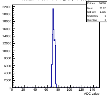
Pedestals mcm83-5A13-refv5-g0-s0-p1 ch 33 test1
