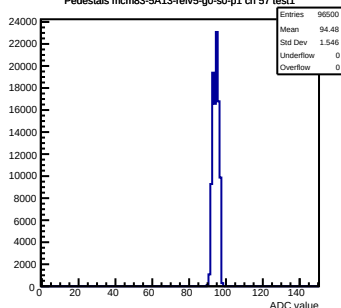
Pedestals mcm83-5A13-refV5-g0-s0-p1 ch 57 test1
