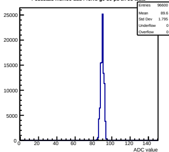
Pedestals mcm90-2214-refv1-g0-s0-p1 ch 98 test1
