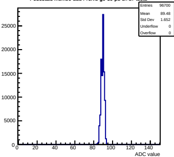
Pedestals mcm90-2214-refv1-g0-s0-p1 ch 17 test1
