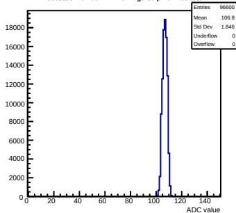
Pedestals mcm90-2214-refv1-g0-s0-p1 ch 106 test1
