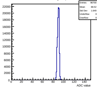
Pedestals mcm90-2214-refv1-g0-s0-p1 ch 30 test1
