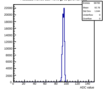
Pedestals mcm90-2214-refv1-g0-s0-p1 ch 19 test1
