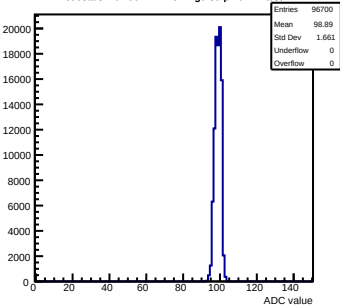
Pedestals mcm90-2214-refv1-g0-s0-p1 ch 21 test1
