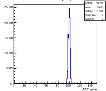
Pedestals mcm90-2214-refv1-g0-s0-p1 ch 23 test1
