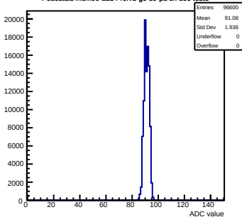
Pedestals mcm90-2214-refv1-g0-s0-p1 ch 96 test1
