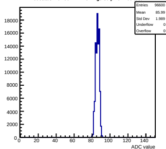
Pedestals mcm90-2214-refv1-g0-s0-p1 ch 109 test1
