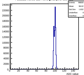
Pedestals mcm90-2214-refv1-g0-s0-p1 ch 101 test1
