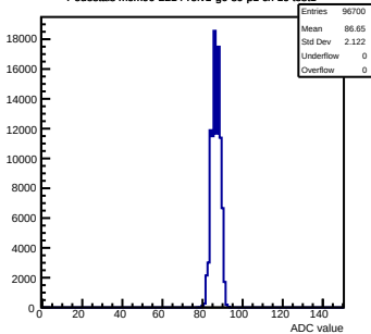
Pedestals mcm90-2214-refv1-g0-s0-p1 ch 16 test1
