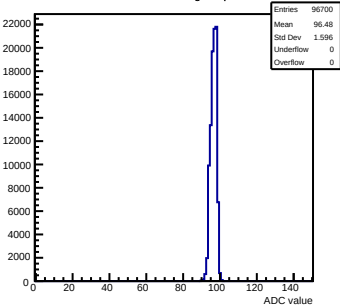
Pedestals mcm90-2214-refv1-g0-s0-p1 ch 29 test1
