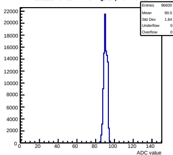
Pedestals mcm90-2214-refv1-g0-s0-p1 ch 110 test1
