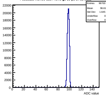
Pedestals mcm90-2214-refv1-g0-s0-p1 ch 18 test1
