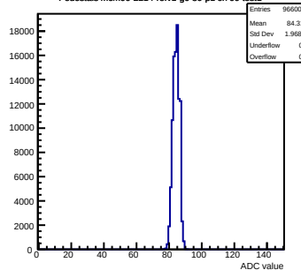
Pedestals mcm90-2214-refv1-g0-s0-p1 ch 99 test1
