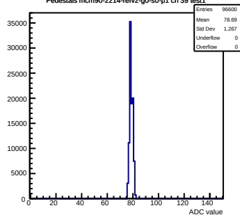
Pedestals mcm90-2214-refv2-g0-s0-p1 ch 39 test1
