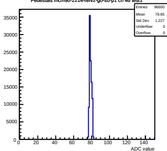
Pedestals mcm90-2214-refv2-g0-s0-p1 ch 46 test1
