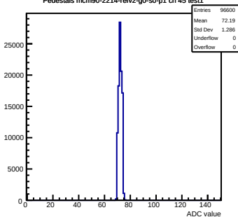
Pedestals mcm90-2214-refv2-g0-s0-p1 ch 45 test1
