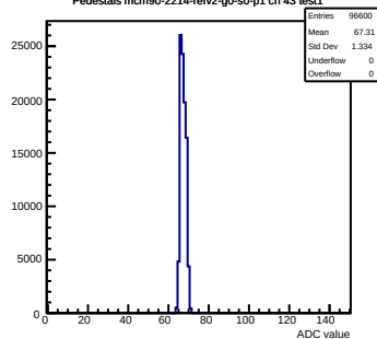
Pedestals mcm90-2214-refv2-g0-s0-p1 ch 43 test1
