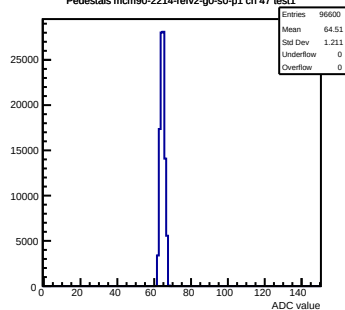
Pedestals mcm90-2214-refv2-g0-s0-p1 ch 47 test1
