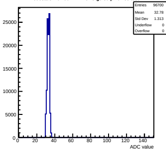
Pedestals mcm90-2214-refv3-g0-s0-p1 ch 88 test1
