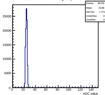
Pedestals mcm90-2214-refv3-g0-s0-p1 ch 91 test1
