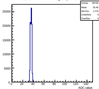
Pedestals mcm90-2214-refv3-g0-s0-p1 ch 95 test1
