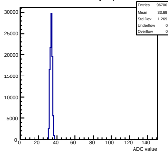
Pedestals mcm90-2214-refv3-g0-s0-p1 ch 89 test1
