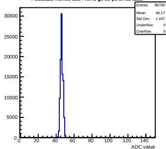
Pedestals mcm90-2214-refv3-g0-s0-p1 ch 82 test1
