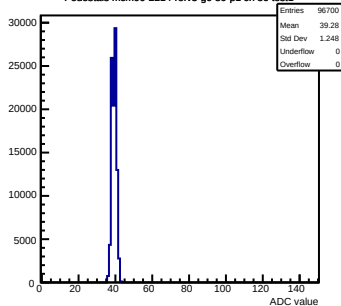
Pedestals mcm90-2214-refv3-g0-s0-p1 ch 86 test1
