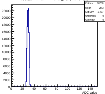
Pedestals mcm90-2214-refv3-g0-s0-p1 ch 84 test1
