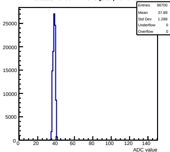
Pedestals mcm90-2214-refv3-g0-s0-p1 ch 92 test1
