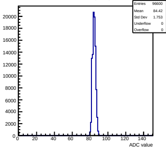
Pedestals mcm90-2214-refV5-g0-s0-p1 ch 100 test1
