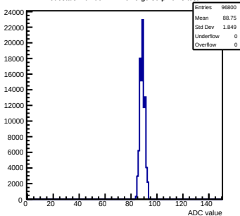
Pedestals mcm90-2214-rvf5-g0-s0-p1 ch 8 test1
