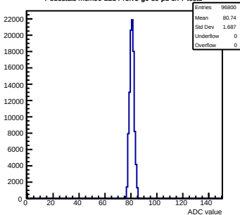
Pedestals mcm90-2214-rvf5-g0-s0-p1 ch 7 test1
