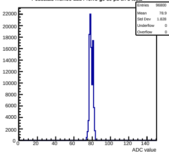
Pedestals mcm90-2214-rvf5-g0-s0-p1 ch 3 test1
