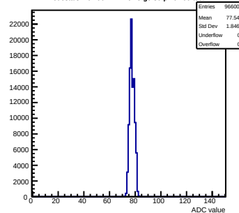
Pedestals mcm90-2214-refV5-g0-s0-p1 ch 99 test1
