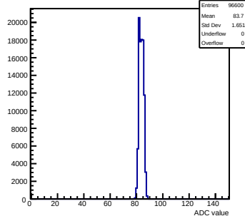
Pedestals mcm90-2214-refV5-g0-s0-p1 ch 110 test1
