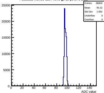
Pedestals mcm90-2214-rvf5-g0-s0-p1 ch 6 test1
