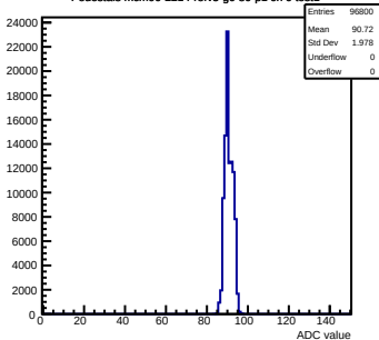
Pedestals mcm90-2214-rvf5-g0-s0-p1 ch 0 test1
