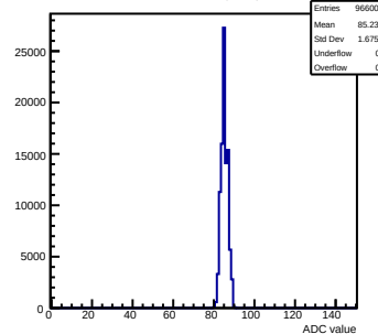
Pedestals mcm90-2214-refV5-g0-s0-p1 ch 103 test1
