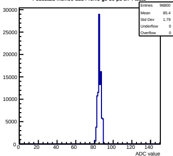
Pedestals mcm90-2214-rvf5-g0-s0-p1 ch 4 test1
