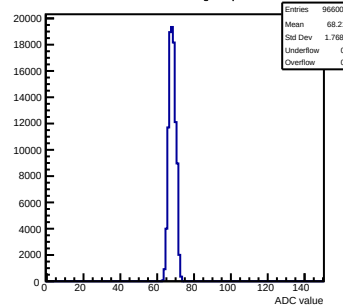
Pedestals mcm90-2214-refV5-g0-s0-p1 ch 107 test1
