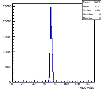
Pedestals mcm90-2214-refV5-g0-s0-p1 ch 102 test1
