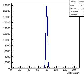
Pedestals mcm90-2214-refV5-g0-s0-p1 ch 111 test1
