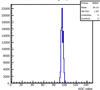
Pedestals mcm90-2214-rvf5-g0-s0-p1 ch 10 test1
