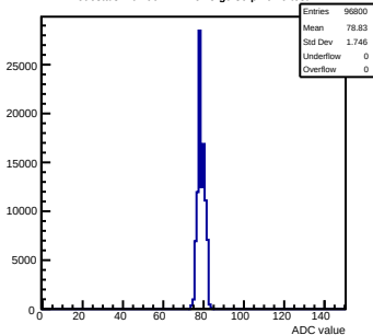
Pedestals mcm90-2214-rvf5-g0-s0-p1 ch 9 test1
