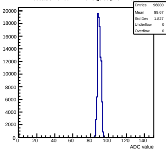
Pedestals mcm90-2214-rvf5-g0-s0-p1 ch 12 test1
