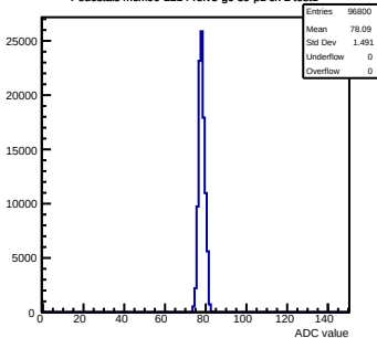
Pedestals mcm90-2214-rvf5-g0-s0-p1 ch 2 test1
