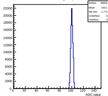
Pedestals mcm90-2214-refV5-g0-s0-p1 ch 106 test1
