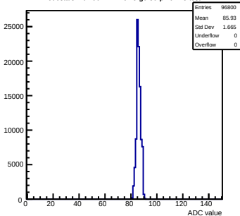
Pedestals mcm90-2214-rvf5-g0-s0-p1 ch 15 test1
