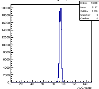
Pedestals mcm90-2214-rvf5-g0-s0-p1 ch 11 test1
