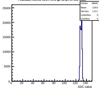
Pedestals mcm90-2214-rlv6-g0-s0-p1 ch 101 test1
