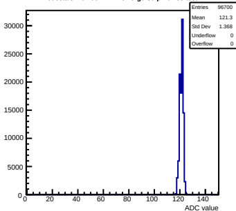
Pedestals mcm90-2214- rev6 -g0-s0-p1 ch 88 test1
