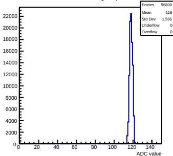
Pedestals mcm90-2214-rlv6-g0-s0-p1 ch 77 test1
