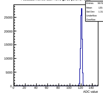
Pedestals mcm90-2214- rev6 -g0-s0-p1 ch 87 test1
