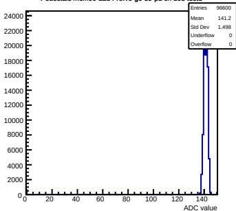
Pedestals mcm90-2214-rlv6-g0-s0-p1 ch 108 test1
