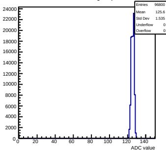
Pedestals mcm90-2214-rlv6-g0-s0-p1 ch 73 test1
