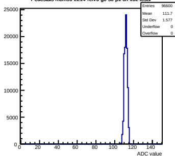
Pedestals mcm90-2214-rlv6-g0-s0-p1 ch 102 test1
