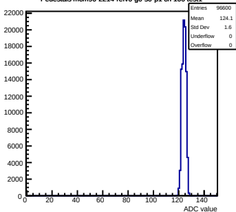
Pedestals mcm90-2214-rlv6-g0-s0-p1 ch 100 test1
