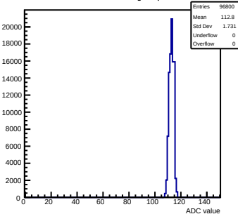
Pedestals mcm90-2214-rlv6-g0-s0-p1 ch 72 test1
