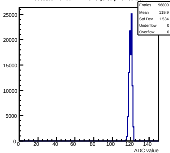
Pedestals mcm90-2214-rlv6-g0-s0-p1 ch 69 test1
