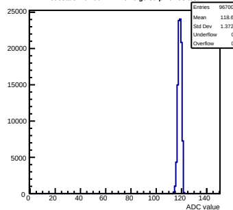
Pedestals mcm90-2214- rev6 -g0-s0-p1 ch 93 test1
