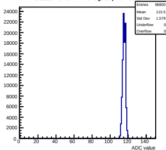
Pedestals mcm90-2214-rlv6-g0-s0-p1 ch 70 test1
