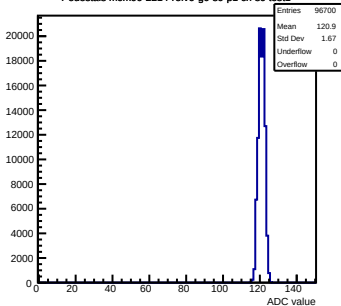
Pedestals mcm90-2214- rev6 -g0-s0-p1 ch 80 test1
