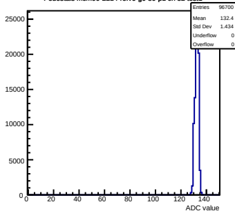
Pedestals mcm90-2214- rev6 -g0-s0-p1 ch 82 test1
