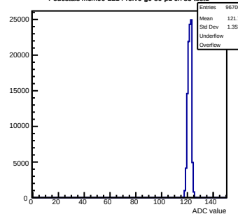
Pedestals mcm90-2214- rev6 -g0-s0-p1 ch 83 test1
