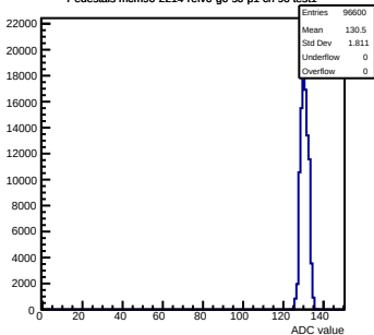
Pedestals mcm90-2214-rlv6-g0-s0-p1 ch 96 test1
