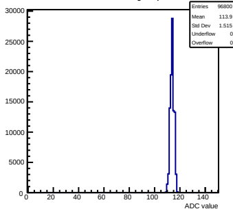
Pedestals mcm90-2214-rlv6-g0-s0-p1 ch 78 test1
