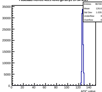
Pedestals mcm91-4611-refV0-g0-s0-p1 ch 94 test1
