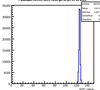
Pedestals mcm91-4611-refV0-g0-s0-p1 ch 93 test1
