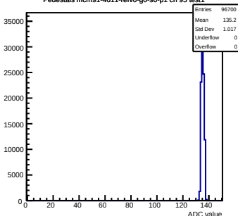
Pedestals mcm91-4611-refV0-g0-s0-p1 ch 95 test1
