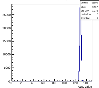
Pedestals mcm91-4611-refV0-g0-s0-p1 ch 45 test1
