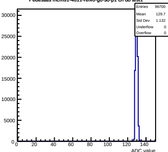
Pedestals mcm91-4611-refV0-g0-s0-p1 ch 88 test1
