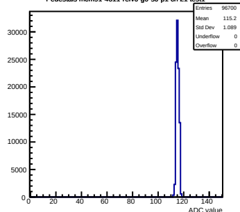
Pedestals mcm91-4611- \text{rev0-g0-s0-p1} ch 21 test1
