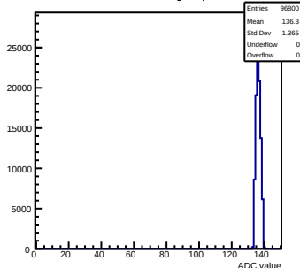
Pedestals mcm91-4611-refV0-g0-s0-p1 ch 73 test1
