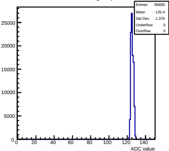
Pedestals mcm91-4611-refV0-g0-s0-p1 ch 43 test1
