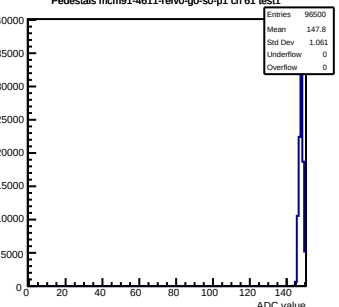
Pedestals mcm91-4611-refV0-g0-s0-p1 ch 61 test1
