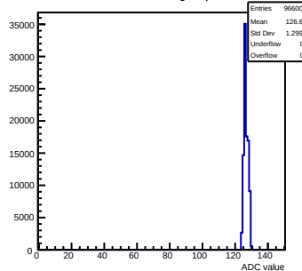
Pedestals mcm91-4611-refV0-g0-s0-p1 ch 46 test1
