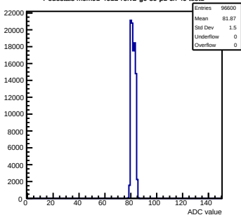
Pedestals mcm91-4611-refv2-g0-s0-p1 ch 40 test1
