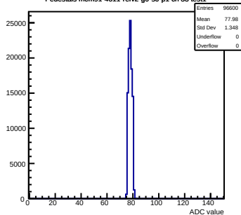
Pedestals mcm91-4611-refv2-g0-s0-p1 ch 33 test1
