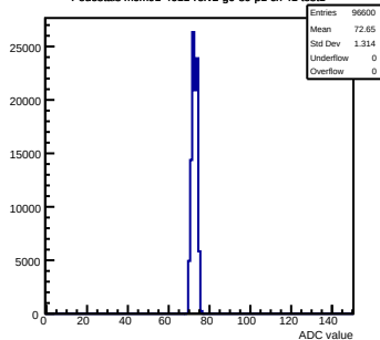
Pedestals mcm91-4611-refv2-g0-s0-p1 ch 41 test1
