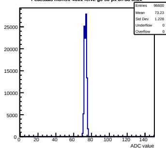
Pedestals mcm91-4611-refv2-g0-s0-p1 ch 38 test1
