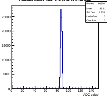
Pedestals mcm91-4611-refv2-g0-s0-p1 ch 32 test1
