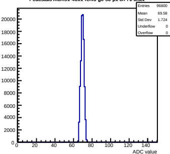
Pedestals mcm91-4611-refV3-g0-s0-p1 ch 71 test1
