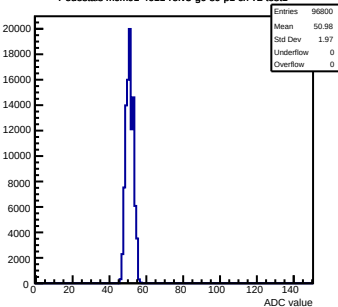
Pedestals mcm91-4611-refV3-g0-s0-p1 ch 72 test1
