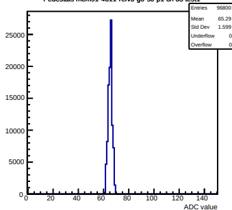
Pedestals mcm91-4611-refV3-g0-s0-p1 ch 65 test1
