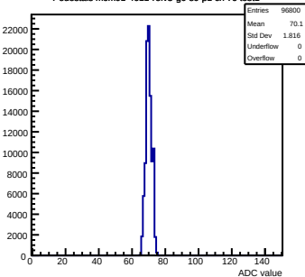
Pedestals mcm91-4611-refV3-g0-s0-p1 ch 76 test1
