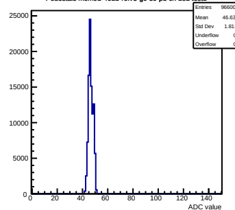
Pedestals mcm91-4611-refv3-g0-s0-p1 ch 102 test1
