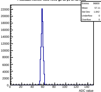
Pedestals mcm91-4611-refV3-g0-s0-p1 ch 68 test1
