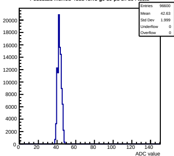
Pedestals mcm91-4611-refv3-g0-s0-p1 ch 104 test1
