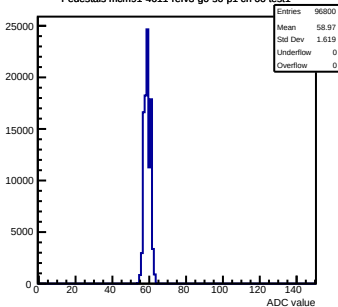
Pedestals mcm91-4611-refV3-g0-s0-p1 ch 66 test1
