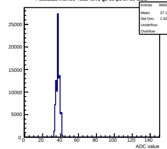
Pedestals mcm91-4611-refv3-g0-s0-p1 ch 99 test1
