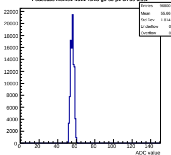
Pedestals mcm91-4611-refV3-g0-s0-p1 ch 69 test1
