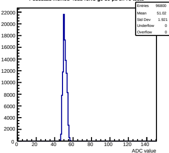
Pedestals mcm91-4611-refV3-g0-s0-p1 ch 79 test1
