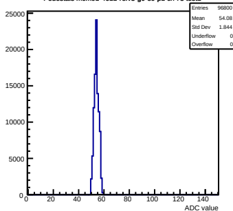
Pedestals mcm91-4611-refV3-g0-s0-p1 ch 73 test1
