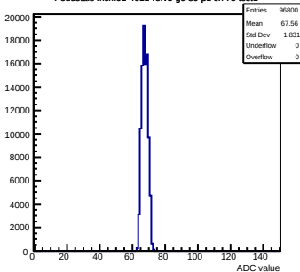
Pedestals mcm91-4611-refV3-g0-s0-p1 ch 78 test1
