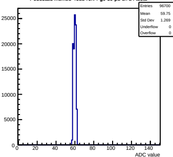
Pedestals mcm91-4611-refv4-g0-s0-p1 ch 24 test1
