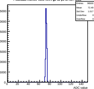
Pedestals mcm91-4611-refv4-g0-s0-p1 ch 117 test1
