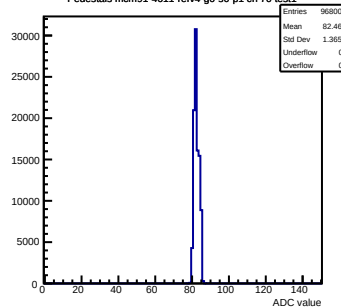
Pedestals mcm91-4611-refV4-g0-s0-p1 ch 70 test1
