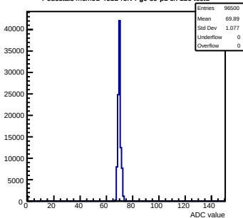
Pedestals mcm91-4611-refv4-g0-s0-p1 ch 120 test1
