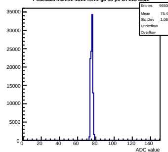
Pedestals mcm91-4611-refv4-g0-s0-p1 ch 115 test1
