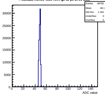
Pedestals mcm91-4611-refv4-g0-s0-p1 ch 21 test1
