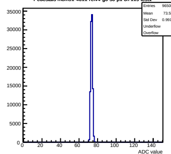
Pedestals mcm91-4611-refv4-g0-s0-p1 ch 119 test1
