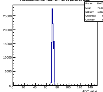
Pedestals mcm91-4611-refv4-g0-s0-p1 ch 39 test1
