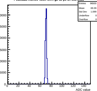
Pedestals mcm91-4611-refv4-g0-s0-p1 ch 113 test1
