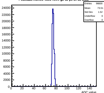
Pedestals mcm91-4611-refv4-g0-s0-p1 ch 36 test1
