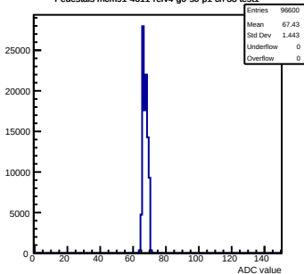
Pedestals mcm91-4611-refv4-g0-s0-p1 ch 33 test1
