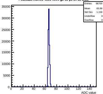
Pedestals mcm91-4611-refv4-g0-s0-p1 ch 18 test1
