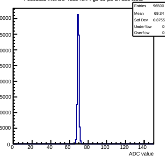
Pedestals mcm91-4611-refv4-g0-s0-p1 ch 121 test1
