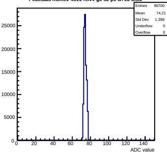
Pedestals mcm91-4611-refv4-g0-s0-p1 ch 20 test1
