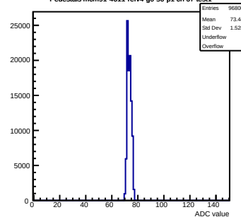
Pedestals mcm91-4611-refV4-g0-s0-p1 ch 67 test1
