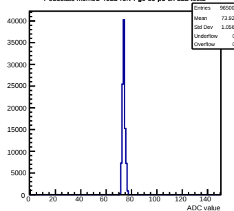
Pedestals mcm91-4611-refv4-g0-s0-p1 ch 122 test1
