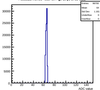
Pedestals mcm91-4611-refv4-g0-s0-p1 ch 29 test1
