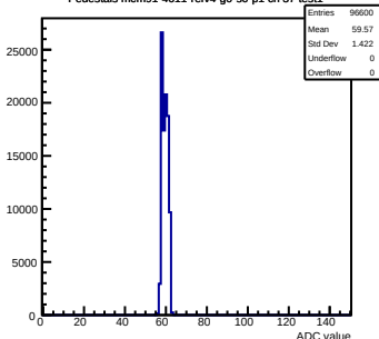
Pedestals mcm91-4611-refv4-g0-s0-p1 ch 37 test1
