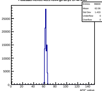
Pedestals mcm91-4611-refv4-g0-s0-p1 ch 44 test1
