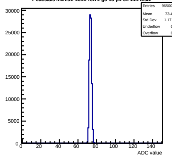
Pedestals mcm91-4611-refv4-g0-s0-p1 ch 114 test1
