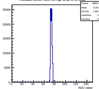
Pedestals mcm91-4611-refV4-g0-s0-p1 ch 69 test1
