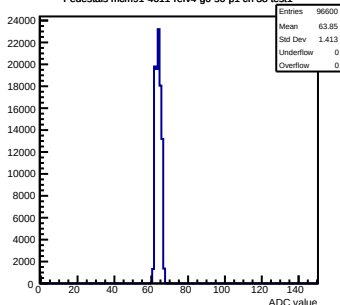
Pedestals mcm91-4611-refv4-g0-s0-p1 ch 38 test1
