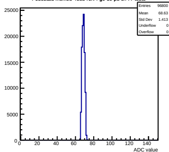
Pedestals mcm91-4611-refV4-g0-s0-p1 ch 77 test1
