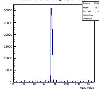
Pedestals mcm91-4611-refv4-g0-s0-p1 ch 123 test1
