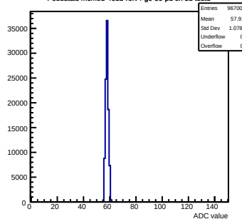
Pedestals mcm91-4611-refv4-g0-s0-p1 ch 31 test1
