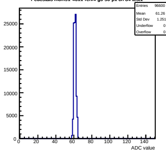
Pedestals mcm91-4611-refv4-g0-s0-p1 ch 34 test1
