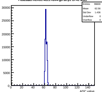
Pedestals mcm91-4611-refv4-g0-s0-p1 ch 41 test1
