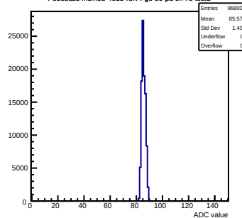
Pedestals mcm91-4611-refV4-g0-s0-p1 ch 78 test1
