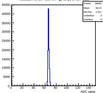
Pedestals mcm91-4611-refv4-g0-s0-p1 ch 124 test1
