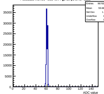
Pedestals mcm91-4611-refv4-g0-s0-p1 ch 27 test1
