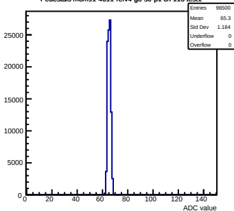
Pedestals mcm91-4611-refv4-g0-s0-p1 ch 116 test1
