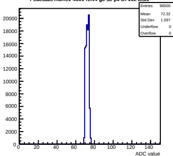
Pedestals mcm91-4611-refv4-g0-s0-p1 ch 112 test1
