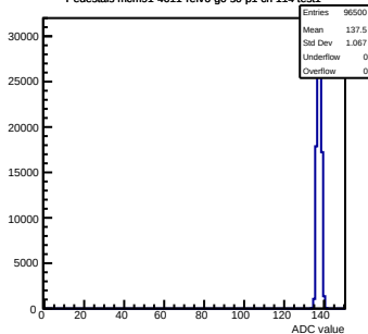
Pedestals mcm91-4611-rlv6-g0-s0-p1 ch 114 test1
