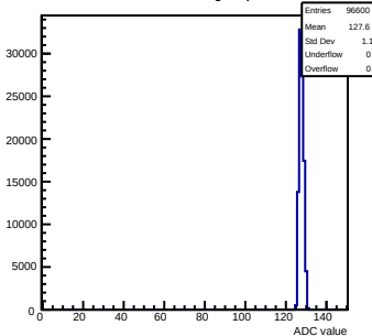
Pedestals mcm91-4611-rlv6-g0-s0-p1 ch 110 test1
