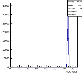
Pedestals mcm91-4611- rfv6-g0-s0-p1 ch 82 test1
