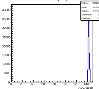
Pedestals mcm91-4611-rlv6-g0-s0-p1 ch 125 test1
