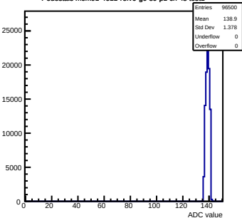
Pedestals mcm91-4611- rfv6-g0-s0-p1 ch 48 test1
