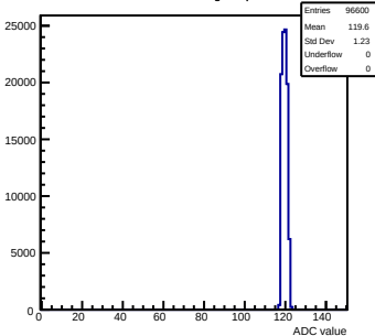
Pedestals mcm91-4611-rlv6-g0-s0-p1 ch 111 test1
