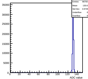
Pedestals mcm91-4611- rfv6-g0-s0-p1 ch 85 test1
