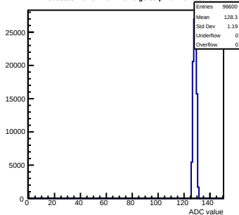
Pedestals mcm91-4611-rlv6-g0-s0-p1 ch 101 test1
