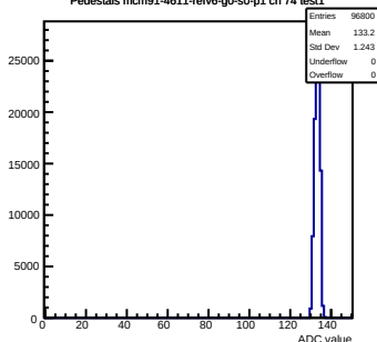
Pedestals mcm91-4611- \nu e6-g0-s0-p1 ch 74 test1
