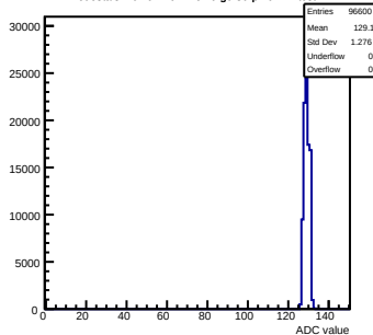
Pedestals mcm91-4611- rfv6-g0-s0-p1 ch 42 test1
