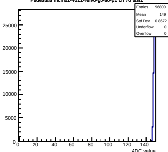
Pedestals mcm91-4611- \nu e6-g0-s0-p1 ch 76 test1
