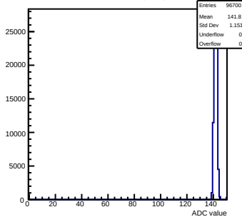
Pedestals mcm91-4611- rfv6-g0-s0-p1 ch 81 test1
