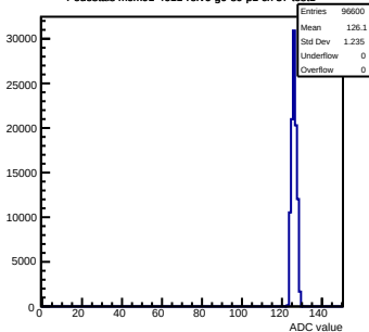
Pedestals mcm91-4611- rfv6-g0-s0-p1 ch 37 test1
