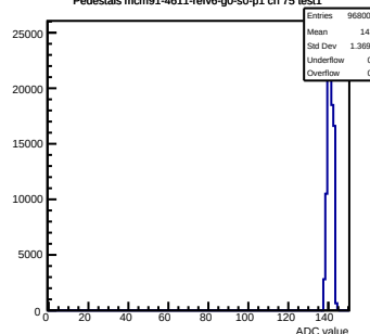
Pedestals mcm91-4611- \nu e6-g0-s0-p1 ch 75 test1
