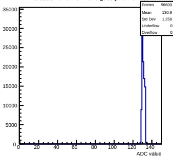
Pedestals mcm91-4611-rlv6-g0-s0-p1 ch 102 test1
