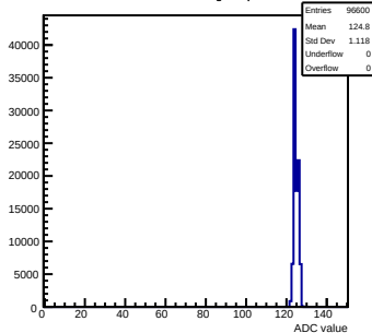
Pedestals mcm91-4611-rlv6-g0-s0-p1 ch 109 test1
