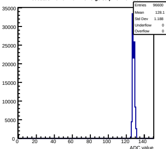
Pedestals mcm91-4611-rlv6-g0-s0-p1 ch 107 test1
