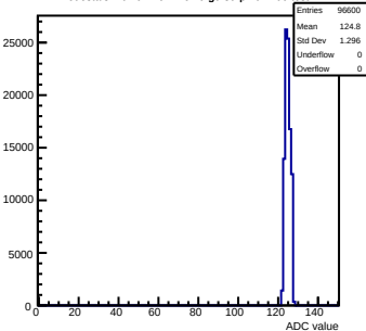
Pedestals mcm91-4611-rlv6-g0-s0-p1 ch 100 test1
