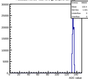
Pedestals mcm91-4611- rfv6-g0-s0-p1 ch 33 test1
