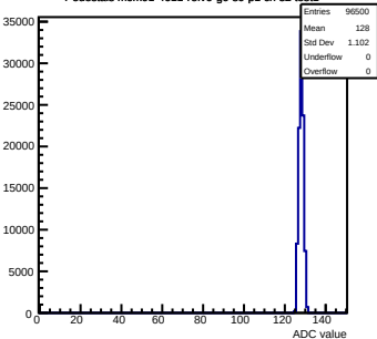
Pedestals mcm91-4611- rfv6-g0-s0-p1 ch 52 test1
