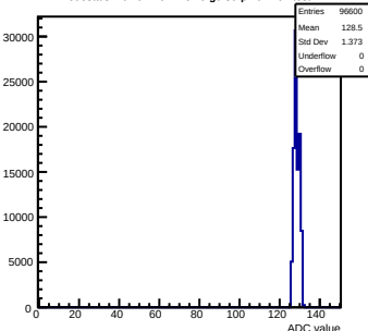
Pedestals mcm91-4611-rlv6-g0-s0-p1 ch 104 test1
