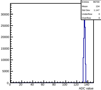
Pedestals mcm91-4611- rfv6-g0-s0-p1 ch 84 test1
