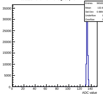
Pedestals mcm91-4611-rlv6-g0-s0-p1 ch 127 test1
