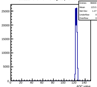
Pedestals mcm91-4611-rlv6-g0-s0-p1 ch 106 test1
