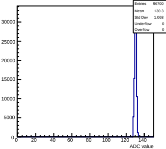
Pedestals mcm91-4611- rfv6-g0-s0-p1 ch 88 test1
