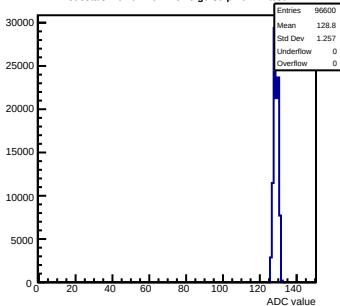
Pedestals mcm91-4611- rfv6-g0-s0-p1 ch 41 test1
