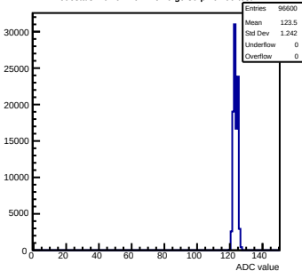
Pedestals mcm91-4611-rlv6-g0-s0-p1 ch 99 test1
