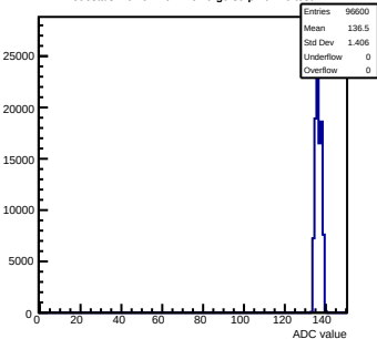
Pedestals mcm91-4611- rfv6-g0-s0-p1 ch 40 test1
