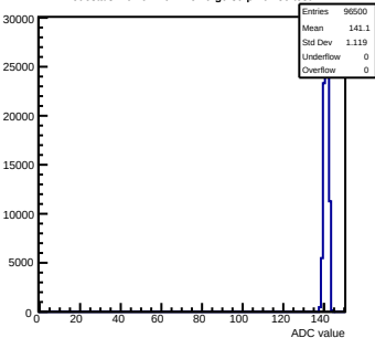
Pedestals mcm91-4611- rfv6-g0-s0-p1 ch 56 test1
