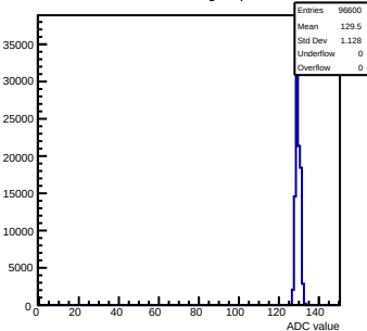
Pedestals mcm91-4611-rlv6-g0-s0-p1 ch 108 test1
