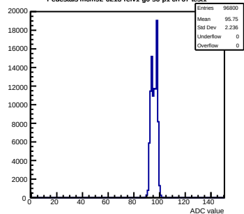
Pedestals mcm92-6213-refv1-g0-s0-p1 ch 67 test1
