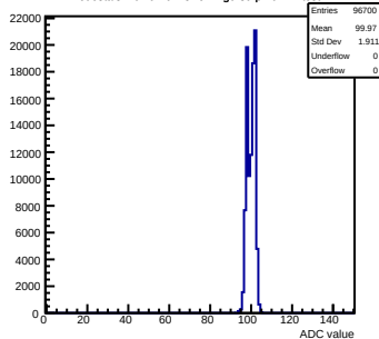
Pedestals mcm92-6213-recv1-g0-s0-p1 ch 17 test1
