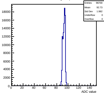
Pedestals mcm92-6213-recv1-g0-s0-p1 ch 28 test1
