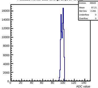
Pedestals mcm92-6213-refv1-g0-s0-p1 ch 48 test1
