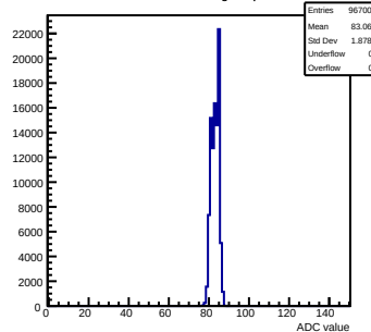
Pedestals mcm92-6213-recv1-g0-s0-p1 ch 27 test1
