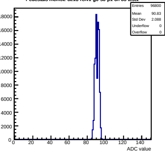
Pedestals mcm92-6213-refv1-g0-s0-p1 ch 65 test1
