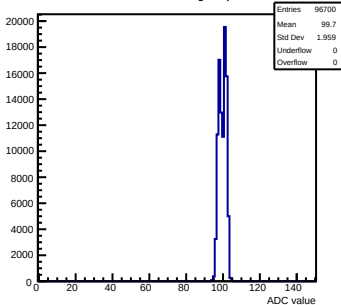
Pedestals mcm92-6213-recv1-g0-s0-p1 ch 20 test1
