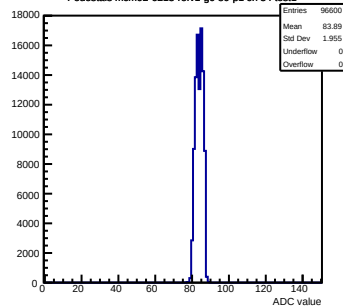
Pedestals mcm92-6213-refv1-g0-s0-p1 ch 34 test1
