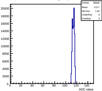
Pedestals mcm92-6213-refv1-g0-s0-p1 ch 63 test1
