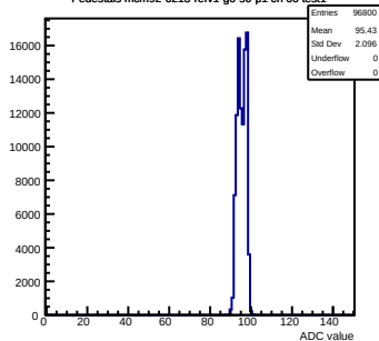
Pedestals mcm92-6213-refv1-g0-s0-p1 ch 66 test1
