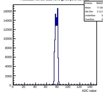
Pedestals mcm92-6213-refv1-g0-s0-p1 ch 38 test1
