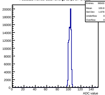
Pedestals mcm92-6213-refv1-g0-s0-p1 ch 49 test1
