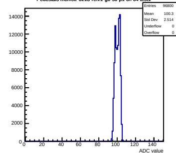
Pedestals mcm92-6213-refv1-g0-s0-p1 ch 64 test1
