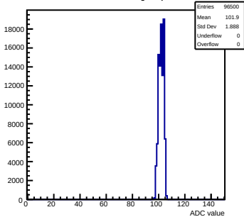
Pedestals mcm92-6213-refv1-g0-s0-p1 ch 56 test1
