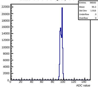
Pedestals mcm92-6213-refv1-g0-s0-p1 ch 52 test1
