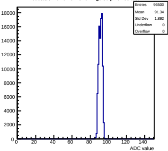
Pedestals mcm92-6213-refv1-g0-s0-p1 ch 55 test1
