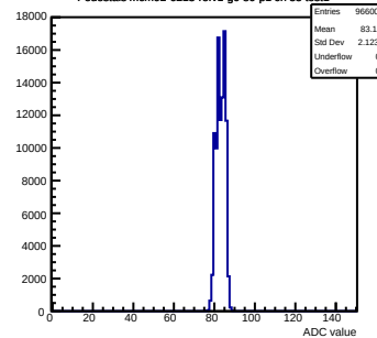
Pedestals mcm92-6213-refv1-g0-s0-p1 ch 35 test1
