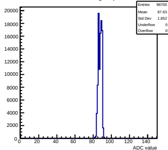
Pedestals mcm92-6213-recv1-g0-s0-p1 ch 25 test1
