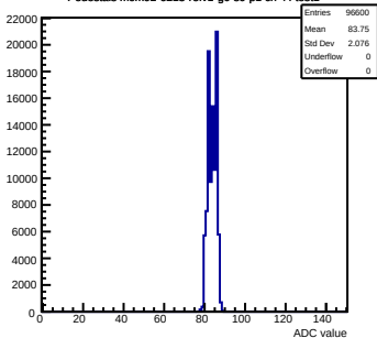
Pedestals mcm92-6213-refv1-g0-s0-p1 ch 44 test1
