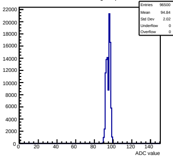
Pedestals mcm92-6213-refv1-g0-s0-p1 ch 58 test1
