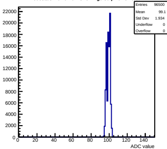
Pedestals mcm92-6213-refv1-g0-s0-p1 ch 54 test1
