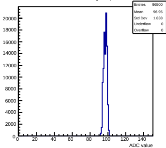
Pedestals mcm92-6213-refv1-g0-s0-p1 ch 60 test1
