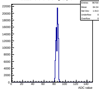
Pedestals mcm92-6213-recv1-g0-s0-p1 ch 22 test1
