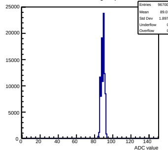
Pedestals mcm92-6213-recv1-g0-s0-p1 ch 23 test1
