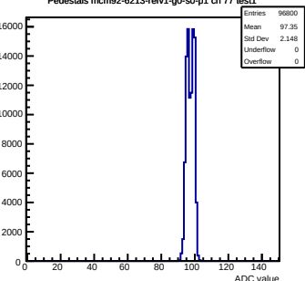
Pedestals mcm92-6213-refv1-g0-s0-p1 ch 77 test1
