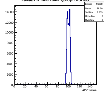
Pedestals mcm92-6213-refv1-g0-s0-p1 ch 68 test1
