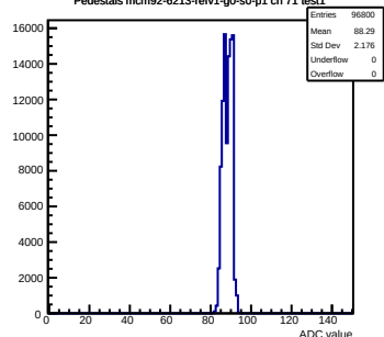
Pedestals mcm92-6213-refv1-g0-s0-p1 ch 71 test1
