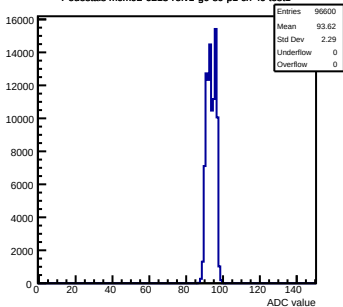
Pedestals mcm92-6213-refv1-g0-s0-p1 ch 40 test1
