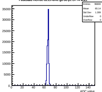
Pedestals mcm92-6213-refv2-g0-s0-p1 ch 74 test1
