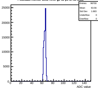
Pedestals mcm92-6213-refv2-g0-s0-p1 ch 80 test1
