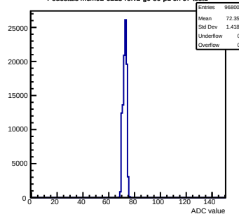
Pedestals mcm92-6213-refv2-g0-s0-p1 ch 67 test1
