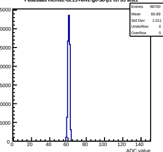
Pedestals mcm92-6213-refv2-g0-s0-p1 ch 93 test1
