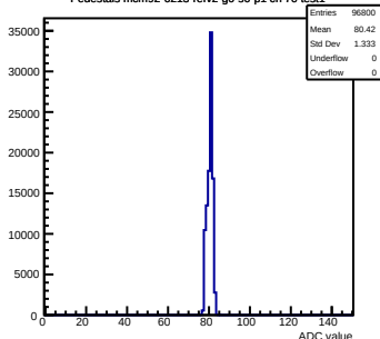
Pedestals mcm92-6213-refv2-g0-s0-p1 ch 70 test1
