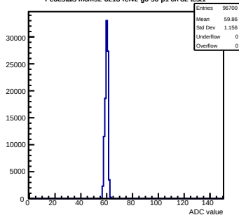
Pedestals mcm92-6213-refv2-g0-s0-p1 ch 82 test1
