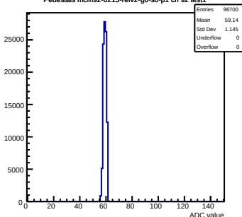
Pedestals mcm92-6213-refv2-g0-s0-p1 ch 92 test1
