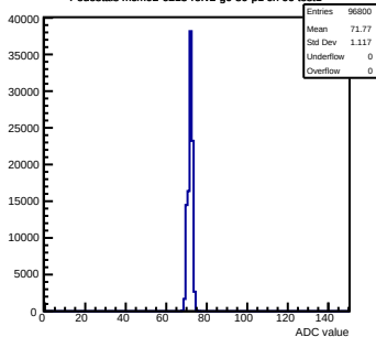
Pedestals mcm92-6213-refv2-g0-s0-p1 ch 66 test1
