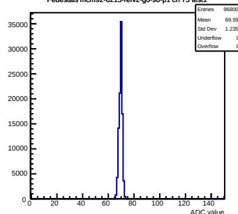
Pedestals mcm92-6213-refv2-g0-s0-p1 ch 75 test1
