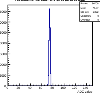
Pedestals mcm92-6213-refv2-g0-s0-p1 ch 85 test1
