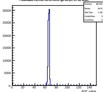
Pedestals mcm92-6213-refv2-g0-s0-p1 ch 90 test1
