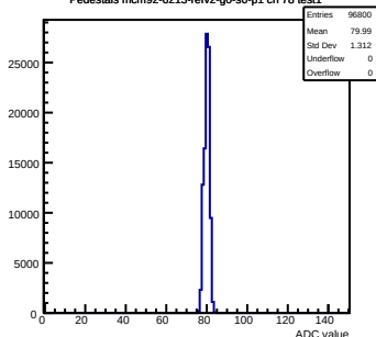
Pedestals mcm92-6213-refv2-g0-s0-p1 ch 78 test1
