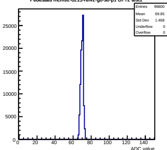
Pedestals mcm92-6213-refv2-g0-s0-p1 ch 72 test1
