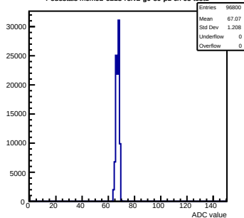
Pedestals mcm92-6213-refv2-g0-s0-p1 ch 65 test1
