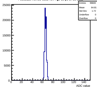
Pedestals mcm92-6213-refv4-g0-s0-p1 ch 33 test1
