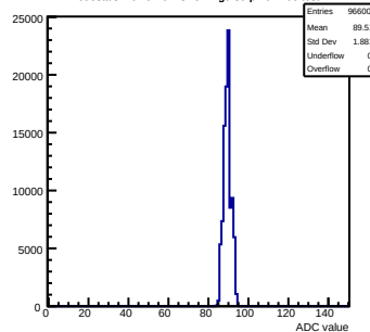
Pedestals mcm92-6213-refv4-g0-s0-p1 ch 106 test1
