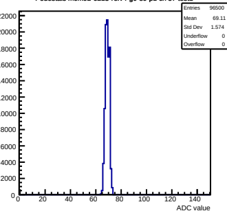
Pedestals mcm92-6213-refv4-g0-s0-p1 ch 57 test1
