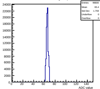
Pedestals mcm92-6213-refv4-g0-s0-p1 ch 45 test1
