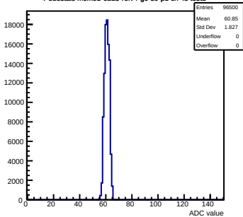
Pedestals mcm92-6213-refv4-g0-s0-p1 ch 48 test1
