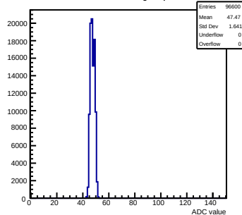
Pedestals mcm92-6213-refv4-g0-s0-p1 ch 46 test1
