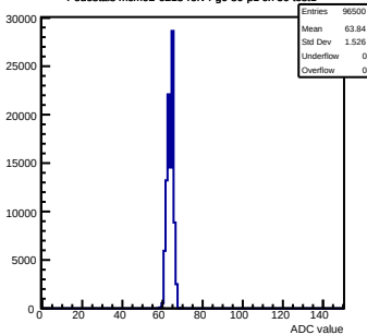
Pedestals mcm92-6213-refv4-g0-s0-p1 ch 50 test1
