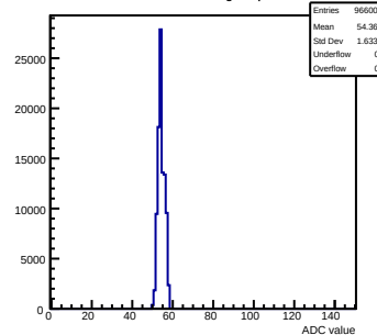
Pedestals mcm92-6213-refv4-g0-s0-p1 ch 47 test1
