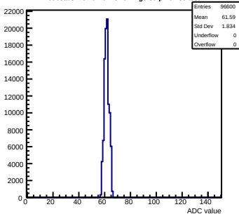
Pedestals mcm92-6213-refv4-g0-s0-p1 ch 36 test1
