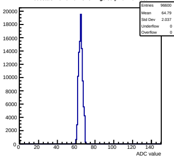
Pedestals mcm92-6213-refv4-g0-s0-p1 ch 104 test1
