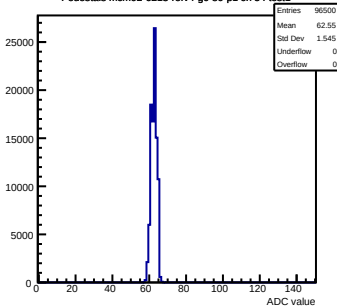
Pedestals mcm92-6213-refv4-g0-s0-p1 ch 54 test1
