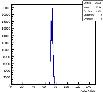
Pedestals mcm92-6213-refv4-g0-s0-p1 ch 108 test1
