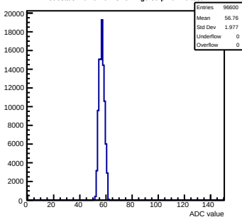
Pedestals mcm92-6213-refv4-g0-s0-p1 ch 40 test1
