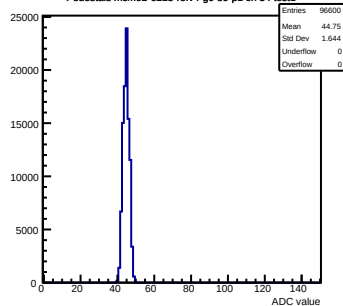
Pedestals mcm92-6213-refv4-g0-s0-p1 ch 34 test1
