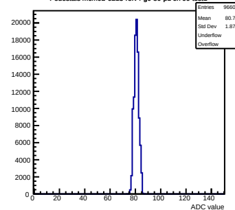
Pedestals mcm92-6213-refv4-g0-s0-p1 ch 99 test1
