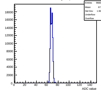
Pedestals mcm92-6213-refv4-g0-s0-p1 ch 111 test1
