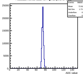
Pedestals mcm92-6213-refv4-g0-s0-p1 ch 97 test1
