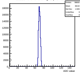
Pedestals mcm92-6213-refv4-g0-s0-p1 ch 105 test1
