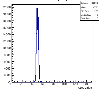
Pedestals mcm92-6213-refv4-g0-s0-p1 ch 41 test1
