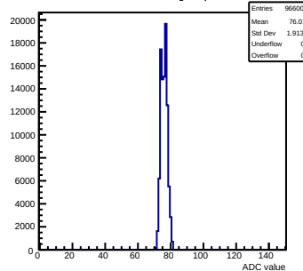
Pedestals mcm92-6213-refv4-g0-s0-p1 ch 110 test1
