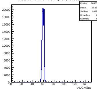
Pedestals mcm92-6213-refv4-g0-s0-p1 ch 59 test1
