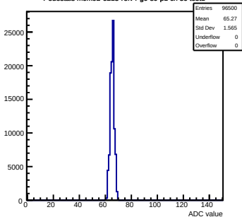
Pedestals mcm92-6213-refv4-g0-s0-p1 ch 56 test1
