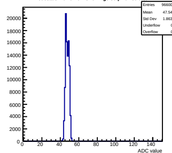
Pedestals mcm92-6213-refv4-g0-s0-p1 ch 39 test1
