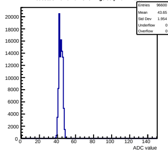
Pedestals mcm92-6213-refv4-g0-s0-p1 ch 42 test1
