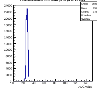
Pedestals mcm93-1215-refv3-g0-s0-p1 ch 79 test1
