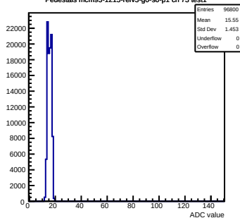
Pedestals mcm93-1215-refv3-g0-s0-p1 ch 73 test1
