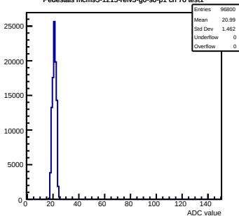
Pedestals mcm93-1215-refv3-g0-s0-p1 ch 76 test1
