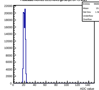
Pedestals mcm93-1215-refv3-g0-s0-p1 ch 75 test1
