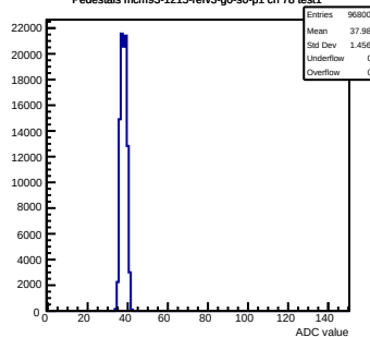
Pedestals mcm93-1215-refv3-g0-s0-p1 ch 78 test1
