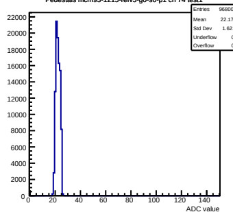
Pedestals mcm93-1215-refv3-g0-s0-p1 ch 74 test1
