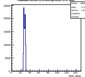
Pedestals mcm93-1215-refv3-g0-s0-p1 ch 67 test1
