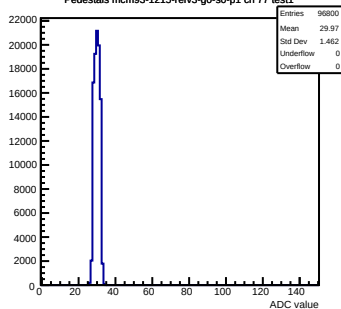
Pedestals mcm93-1215-refv3-g0-s0-p1 ch 77 test1
