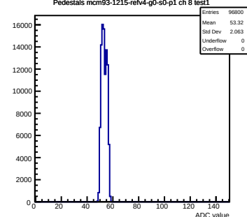
Pedestals mcm93-1215-refv4-g0-s0-p1 ch 8 test1
