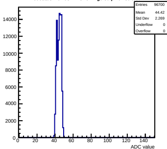
Pedestals mcm93-1215-refv4-g0-s0-p1 ch 80 test1
