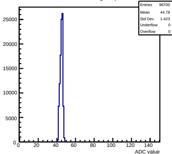
Pedestals mcm93-1215-refv4-g0-s0-p1 ch 93 test1
