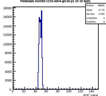
Pedestals mcm93-1215-refv4-g0-s0-p1 ch 10 test1
