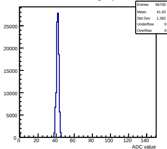
Pedestals mcm93-1215-refv4-g0-s0-p1 ch 95 test1
