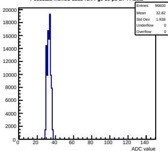
Pedestals mcm93-1215-refv4-g0-s0-p1 ch 44 test1
