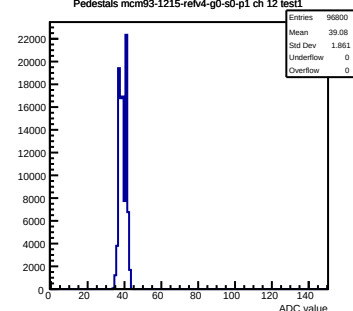
Pedestals mcm93-1215-refv4-g0-s0-p1 ch 12 test1
