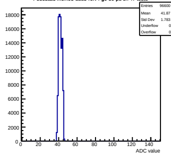
Pedestals mcm93-1215-refv4-g0-s0-p1 ch 47 test1
