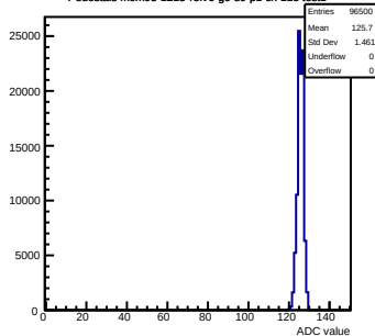
Pedestals mcm93-1215-rlv6-g0-s0-p1 ch 118 test1
