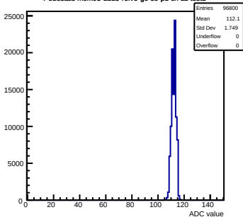
Pedestals mcm93-1215-refv6-g0-s0-p1 ch 12 test1
