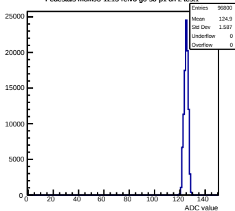
Pedestals mcm93-1215-refv6-g0-s0-p1 ch 2 test1
