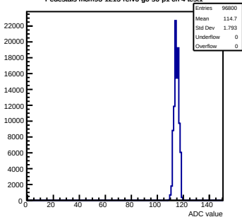
Pedestals mcm93-1215-refv6-g0-s0-p1 ch 4 test1
