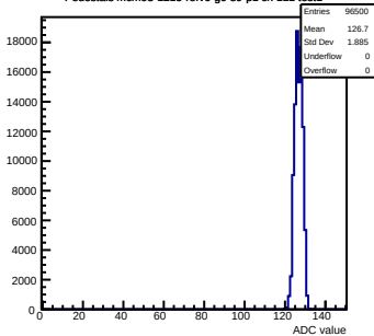
Pedestals mcm93-1215-rlv6-g0-s0-p1 ch 112 test1
