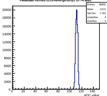
Pedestals mcm93-1215-refv6-g0-s0-p1 ch 74 test1
