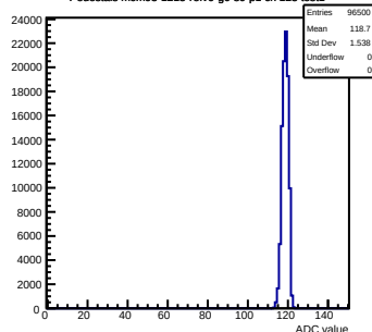
Pedestals mcm93-1215-rlv6-g0-s0-p1 ch 123 test1
