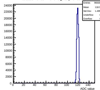
Pedestals mcm93-1215-refv6-g0-s0-p1 ch 55 test1
