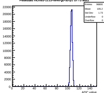
Pedestals mcm93-1215-refv6-g0-s0-p1 ch 73 test1
