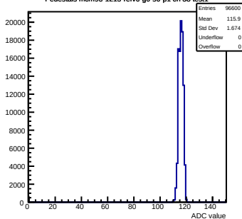
Pedestals mcm93-1215-refv6-g0-s0-p1 ch 38 test1
