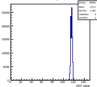
Pedestals mcm93-1215-refv6-g0-s0-p1 ch 56 test1
