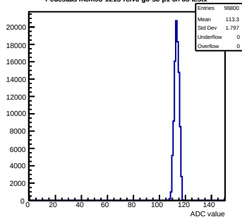
Pedestals mcm93-1215-refv6-g0-s0-p1 ch 65 test1
