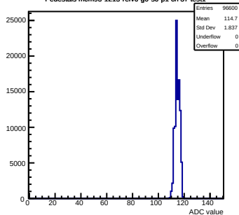
Pedestals mcm93-1215-refv6-g0-s0-p1 ch 37 test1
