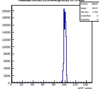
Pedestals mcm93-1215-refv6-g0-s0-p1 ch 70 test1
