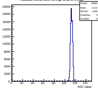
Pedestals mcm93-1215-refv6-g0-s0-p1 ch 3 test1
