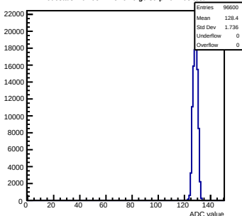
Pedestals mcm93-1215-refv6-g0-s0-p1 ch 108 test1
