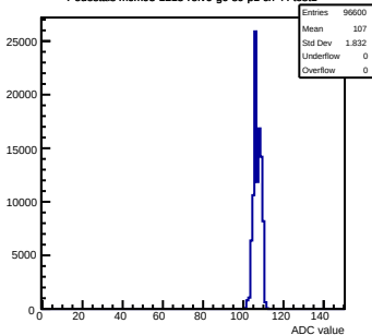
Pedestals mcm93-1215-refv6-g0-s0-p1 ch 44 test1
