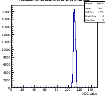
Pedestals mcm93-1215-refv6-g0-s0-p1 ch 32 test1
