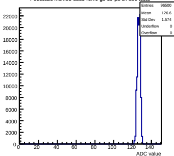
Pedestals mcm93-1215-rlv6-g0-s0-p1 ch 116 test1
