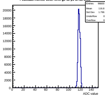
Pedestals mcm93-1215-refv6-g0-s0-p1 ch 33 test1
