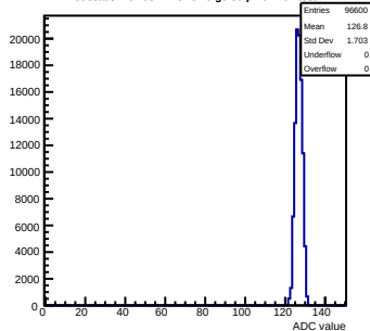
Pedestals mcm93-1215-refv6-g0-s0-p1 ch 101 test1
