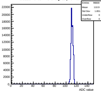
Pedestals mcm93-1215-refv6-g0-s0-p1 ch 96 test1
