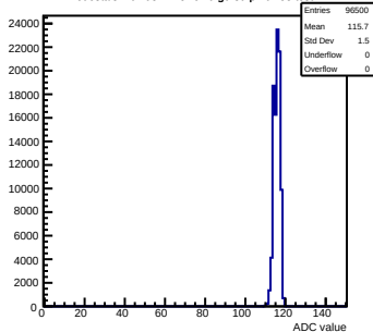
Pedestals mcm93-1215-refv6-g0-s0-p1 ch 53 test1
