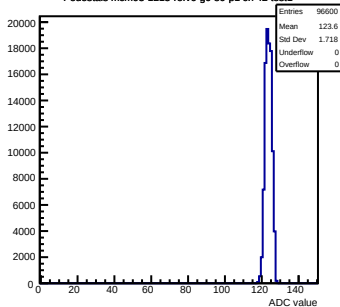
Pedestals mcm93-1215-refv6-g0-s0-p1 ch 42 test1
