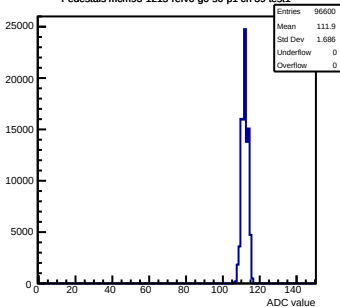
Pedestals mcm93-1215-refv6-g0-s0-p1 ch 39 test1
