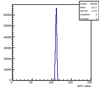
Pedestals mcm 0 ch 29 chamber-fec0
