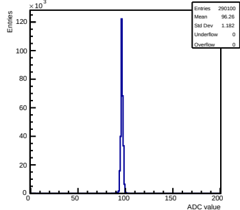
Pedestals mcm 0 ch 17 chamber-fec0
