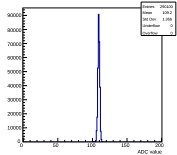
Pedestals mcm 0 ch 83 chamber-fec0
