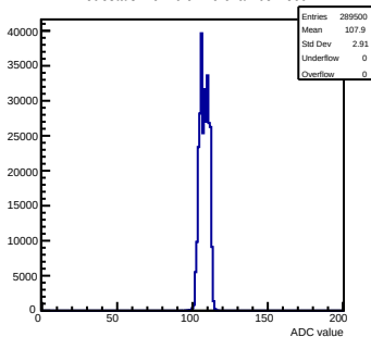
Pedestals mcm 0 ch 49 chamber-fec0
