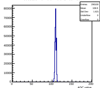
Pedestals mcm 0 ch 26 chamber-fec0
