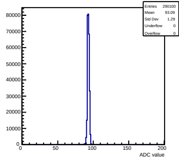
Pedestals mcm 0 ch 19 chamber-fec0
