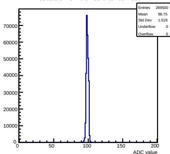
Pedestals mcm 0 ch 53 chamber-fec0
