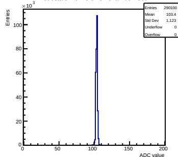
Pedestals mcm 0 ch 94 chamber-fec0
