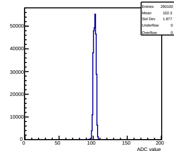
Pedestals mcm 0 ch 28 chamber-fec0
