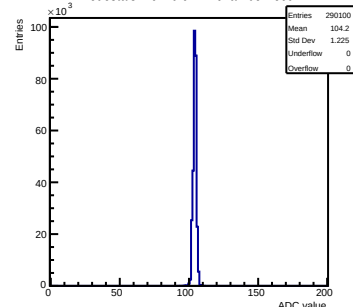
Pedestals mcm 0 ch 24 chamber-fec0
