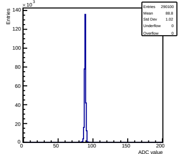
Pedestals mcm 0 ch 87 chamber-fec0
