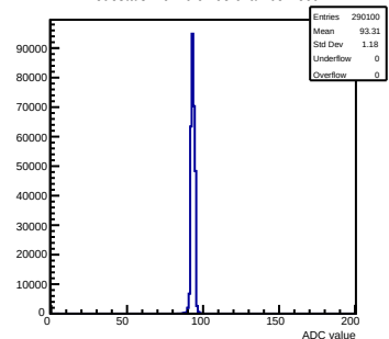
Pedestals mcm 0 ch 95 chamber-fec0
