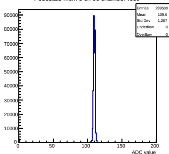
Pedestals mcm 0 ch 60 chamber-fec0
