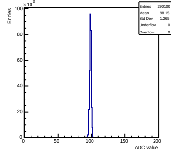
Pedestals mcm 0 ch 20 chamber-fec0
