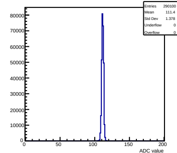
Pedestals mcm 0 ch 16 chamber-fec0
