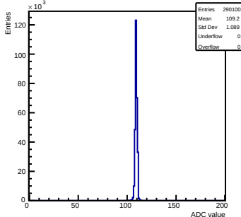
Pedestals mcm 0 ch 85 chamber-fec0
