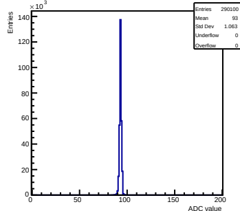
Pedestals mcm 0 ch 86 chamber-fec0
