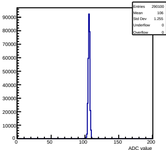
Pedestals mcm 0 ch 84 chamber-fec0
