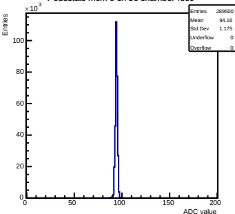
Pedestals mcm 0 ch 56 chamber-fec0
