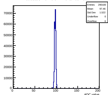
Pedestals mcm 0 ch 27 chamber-fec0
