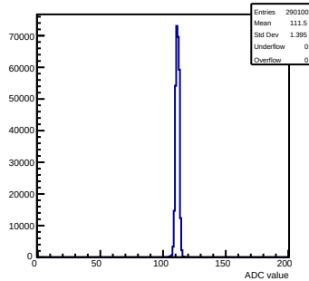
Pedestals mcm 0 ch 81 chamber-fec0
