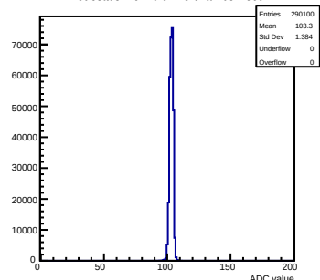
Pedestals mcm 0 ch 25 chamber-fec0
