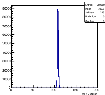
Pedestals mcm 0 ch 54 chamber-fec0
