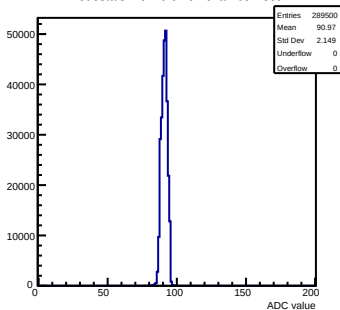
Pedestals mcm 0 ch 51 chamber-fec0
