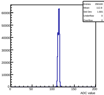
Pedestals mcm 0 ch 80 chamber-fec0
