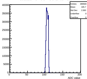
Pedestals mcm 0 ch 48 chamber-fec0
