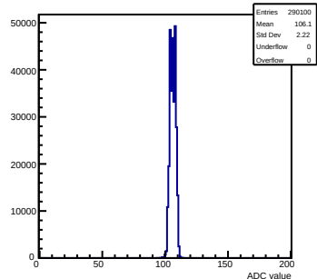
Pedestals mcm 0 ch 31 chamber-fec0
