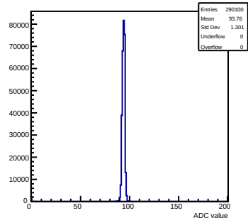
Pedestals mcm 0 ch 21 chamber-fec0
