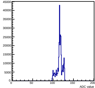
Pedestals mcm 1 ch 55 chamber-fec01
