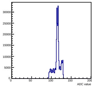
Pedestals mcm 1 ch 107 chamber-fec01
