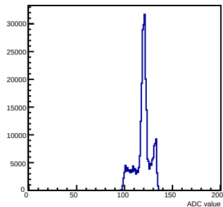
Pedestals mcm 1 ch 47 chamber-fec01
