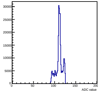
Pedestals mcm 1 ch 62 chamber-fec01
