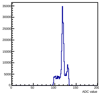
Pedestals mcm 1 ch 68 chamber-fec01
