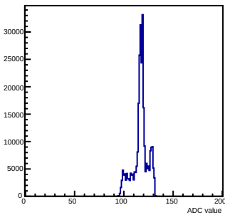
Pedestals mcm 1 ch 100 chamber-fec01
