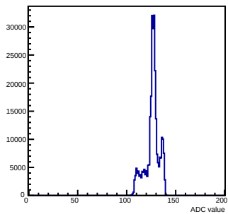
Pedestals mcm 1 ch 17 chamber-fec01
