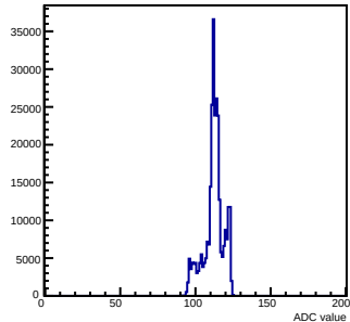
Pedestals mcm 1 ch 63 chamber-fec01
