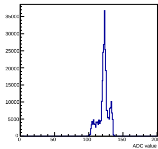
Pedestals mcm 1 ch 18 chamber-fec01
