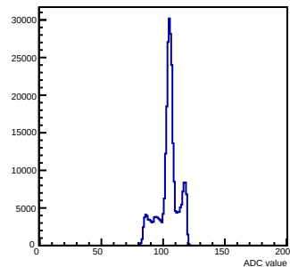
Pedestals mcm 1 ch 79 chamber-fec01
