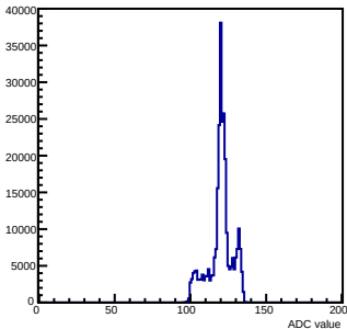
Pedestals mcm 1 ch 40 chamber-fec01
