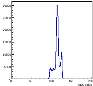
Pedestals mcm 1 ch 57 chamber-fec01
