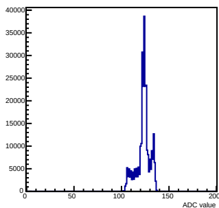
Pedestals mcm 1 ch 4 chamber-fec01
