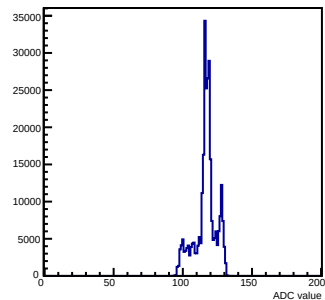
Pedestals mcm 1 ch 95 chamber-fec01
