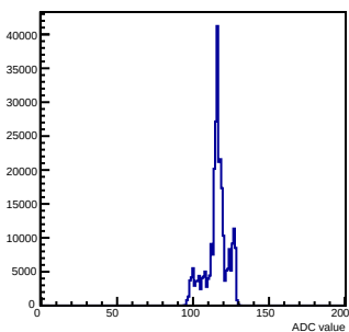
Pedestals mcm 1 ch 13 chamber-fec01
