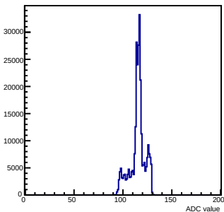
Pedestals mcm 1 ch 44 chamber-fec01
