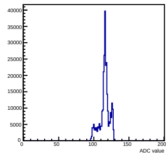
Pedestals mcm 1 ch 27 chamber-fec01
