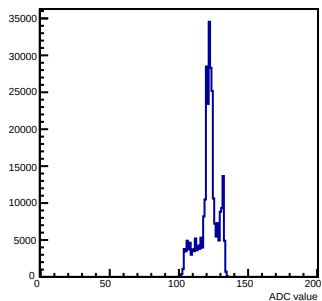
Pedestals mcm 1 ch 29 chamber-fec01
