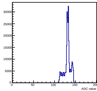
Pedestals mcm 1 ch 114 chamber-fec01
