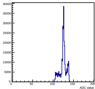
Pedestals mcm 1 ch 121 chamber-fec01
