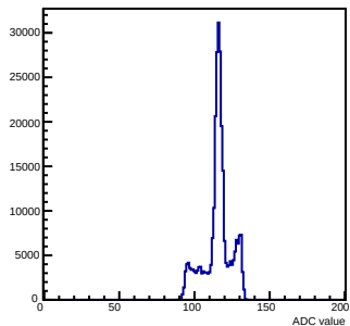
Pedestals mcm 1 ch 77 chamber-fec01
