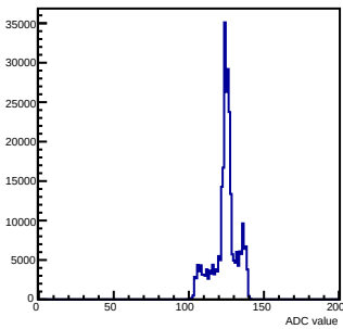
Pedestals mcm 1 ch 96 chamber-fec01
