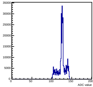
Pedestals mcm 1 ch 81 chamber-fec01
