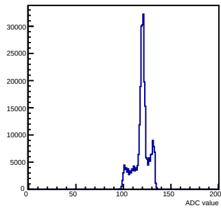
Pedestals mcm 1 ch 99 chamber-fec01
