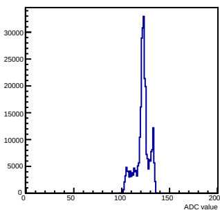
Pedestals mcm 1 ch 5 chamber-fec01
