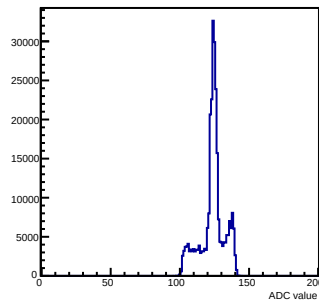
Pedestals mcm 1 ch 106 chamber-fec01
