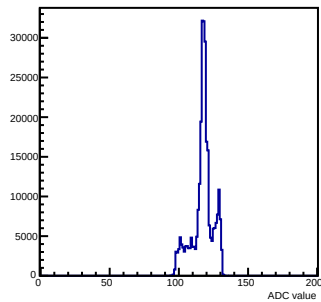
Pedestals mcm 1 ch 34 chamber-fec01
