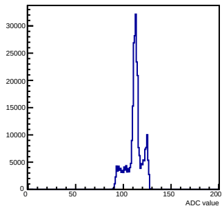
Pedestals mcm 1 ch 69 chamber-fec01
