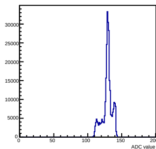
Pedestals mcm 1 ch 6 chamber-fec01
