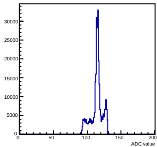
Pedestals mcm 1 ch 33 chamber-fec01
