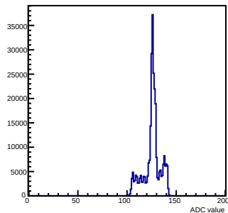
Pedestals mcm 1 ch 74 chamber-fec01
