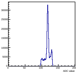
Pedestals mcm 1 ch 36 chamber-fec01
