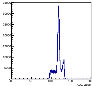
Pedestals mcm 1 ch 70 chamber-fec01
