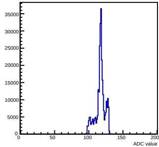
Pedestals mcm 1 ch 51 chamber-fec01
