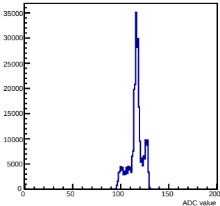
Pedestals mcm 1 ch 52 chamber-fec01
