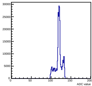
Pedestals mcm 1 ch 65 chamber-fec01
