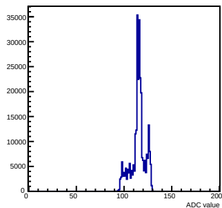
Pedestals mcm 1 ch 125 chamber-fec01
