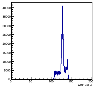
Pedestals mcm 1 ch 109 chamber-fec01
