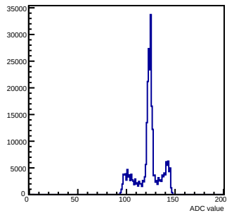
Pedestals mcm 1 ch 89 chamber-fec01
