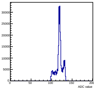
Pedestals mcm 1 ch 84 chamber-fec01
