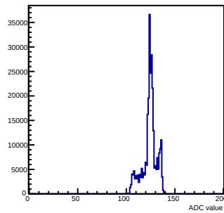
Pedestals mcm 1 ch 98 chamber-fec01
