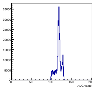
Pedestals mcm 1 ch 14 chamber-fec01
