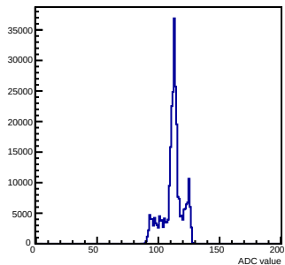
Pedestals mcm 1 ch 45 chamber-fec01
