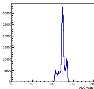
Pedestals mcm 1 ch 10 chamber-fec01
