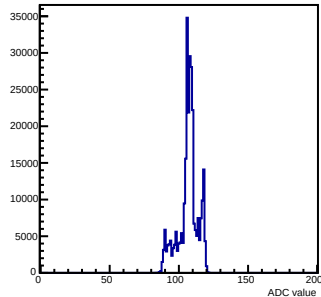
Pedestals mcm 1 ch 58 chamber-fec01
