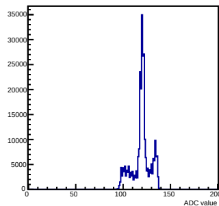
Pedestals mcm 1 ch 118 chamber-fec01
