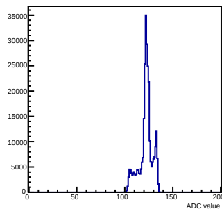
Pedestals mcm 1 ch 30 chamber-fec01
