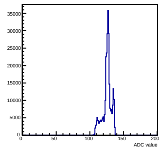
Pedestals mcm 1 ch 23 chamber-fec01
