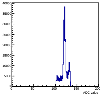
Pedestals mcm 1 ch 116 chamber-fec01
