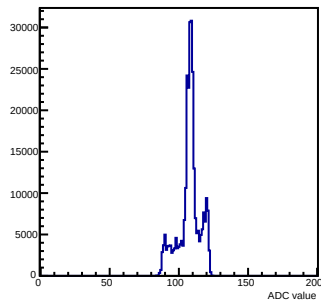
Pedestals mcm 1 ch 42 chamber-fec01
