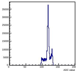
Pedestals mcm 1 ch 73 chamber-fec01
