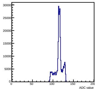
Pedestals mcm 1 ch 78 chamber-fec01
