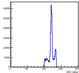
Pedestals mcm 1 ch 87 chamber-fec01
