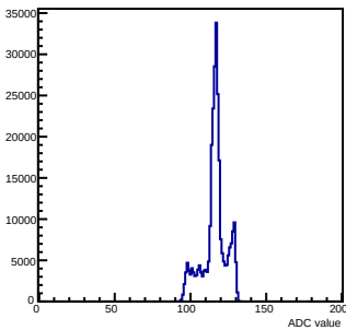
Pedestals mcm 1 ch 108 chamber-fec01
