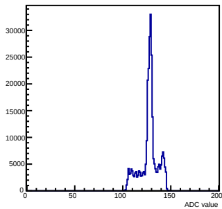
Pedestals mcm 1 ch 64 chamber-fec01
