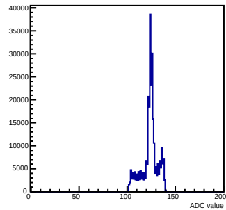
Pedestals mcm 1 ch 67 chamber-fec01
