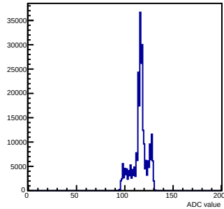
Pedestals mcm 1 ch 50 chamber-fec01
