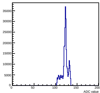
Pedestals mcm 1 ch 21 chamber-fec01
