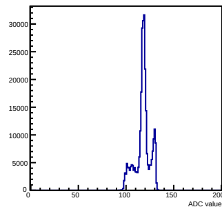
Pedestals mcm 1 ch 119 chamber-fec01
