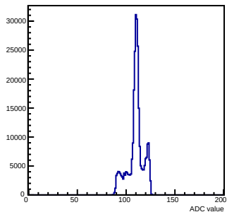
Pedestals mcm 1 ch 41 chamber-fec01
