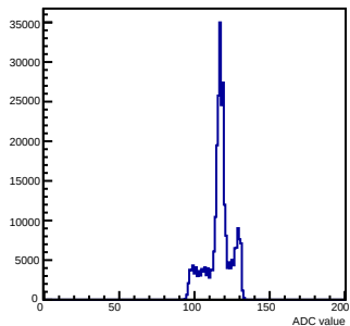
Pedestals mcm 1 ch 37 chamber-fec01
