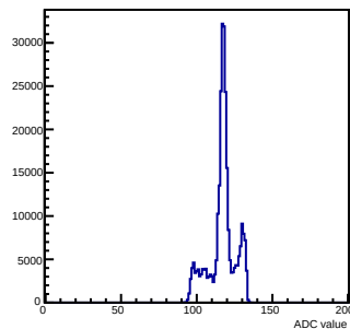
Pedestals mcm 1 ch 122 chamber-fec01
