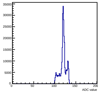
Pedestals mcm 1 ch 113 chamber-fec01
