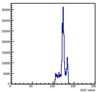
Pedestals mcm 1 ch 1 chamber-fec01
