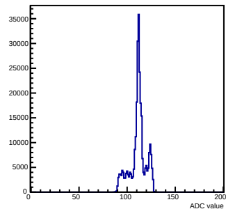
Pedestals mcm 1 ch 71 chamber-fec01
