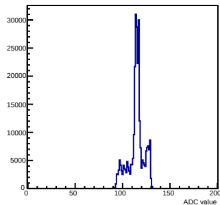
Pedestals mcm 1 ch 46 chamber-fec01
