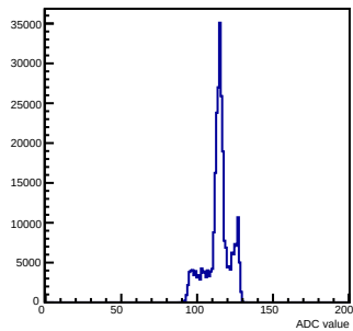
Pedestals mcm 1 ch 111 chamber-fec01
