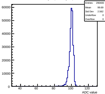
Pedestals chamber-fec01-debug-cik0-ped0-rv0-g0-s0-p1-1008 ch 205 test
