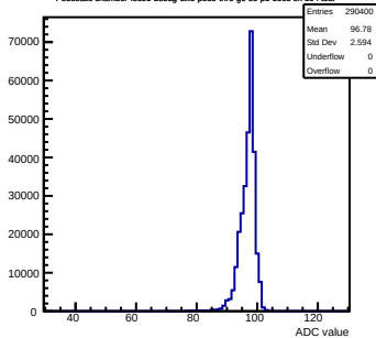
Pedestals chamber-fec01-debug-cik0-ped0-rv0-g0-s0-p1-1008 ch 194 test
