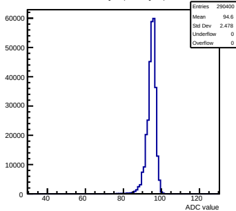
Pedestals chamber-fec01-debug-cik0-ped0-rv0-g0-s0-p1-1008 ch 206 test
