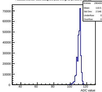
Pedestals chamber-fec01-debug-cik0-ped0-rv0-g0-s0-p1-1008 ch 195 test
