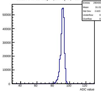
Pedestals chamber-fec01-debug-cik0-ped0-rv0-g0-s0-p1-1008 ch 199 test
