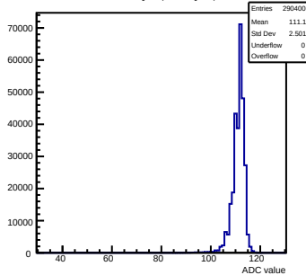
Pedestals chamber-fec01-debug-cik0-ped0-rv0-g0-s0-p1-1008 ch 203 test
