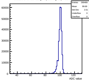
Pedestals chamber-fec01-debug-cik0-ped0-rv0-g0-s0-p1-1008 ch 196 test
