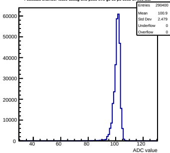
Pedestals chamber-fec01-debug-cik0-ped0-rv0-g0-s0-p1-1008 ch 193 test
