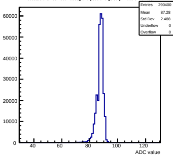
Pedestals chamber-fec01-debug-cik0-ped0-rv0-g0-s0-p1-1008 ch 197 test
