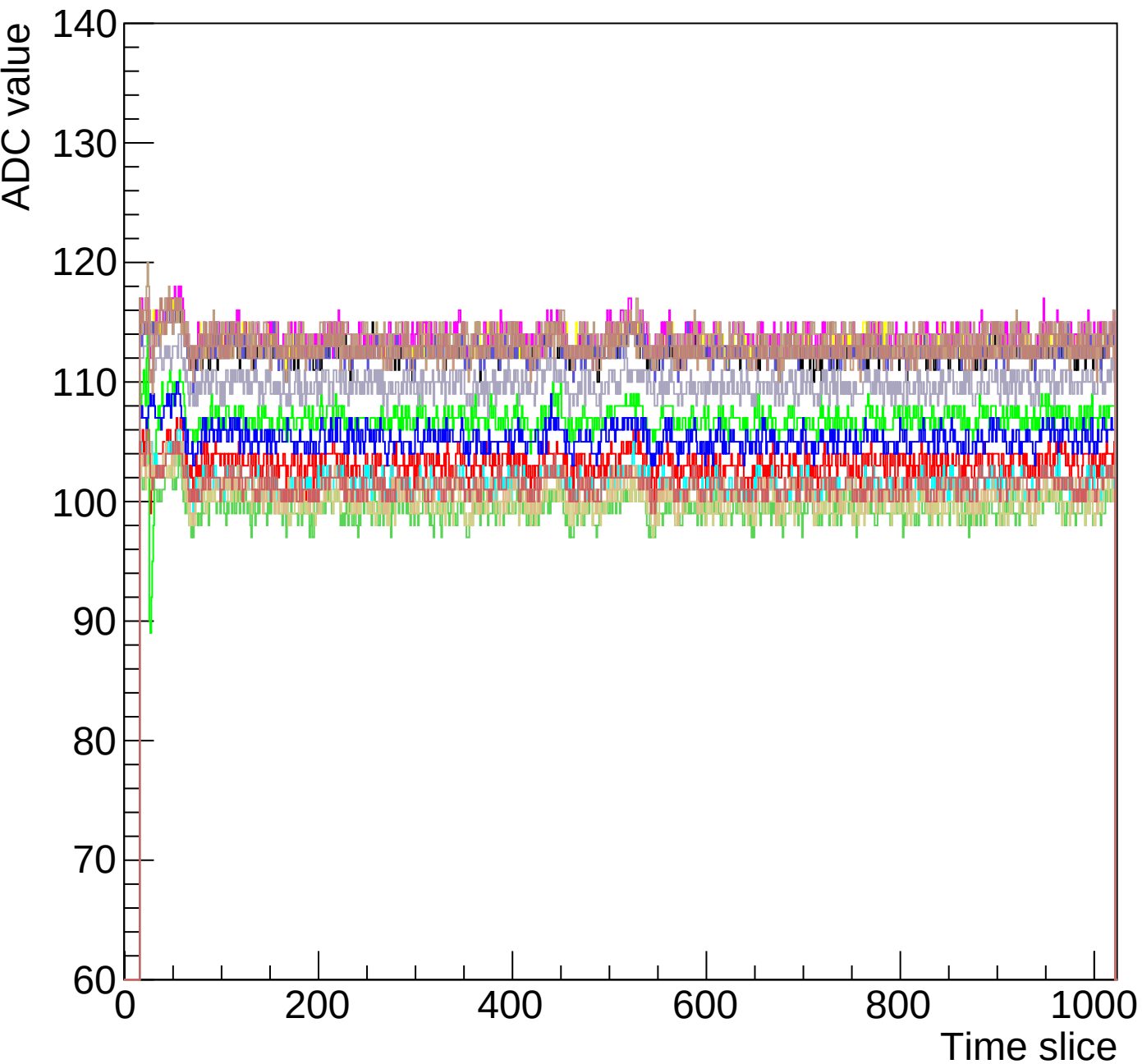
Run 0 event 20 mcm 0 chip 6 chamber-fec01-debug1
