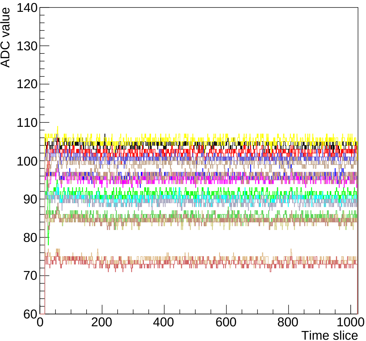
Run 0 event 11 mcm 1 chip 2 plane-fec01-debug
