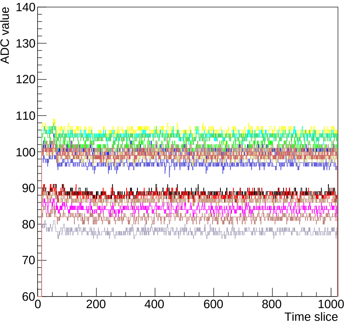
Run 0 event 13 mcm 1 chip 4 plane-fec01-debug
