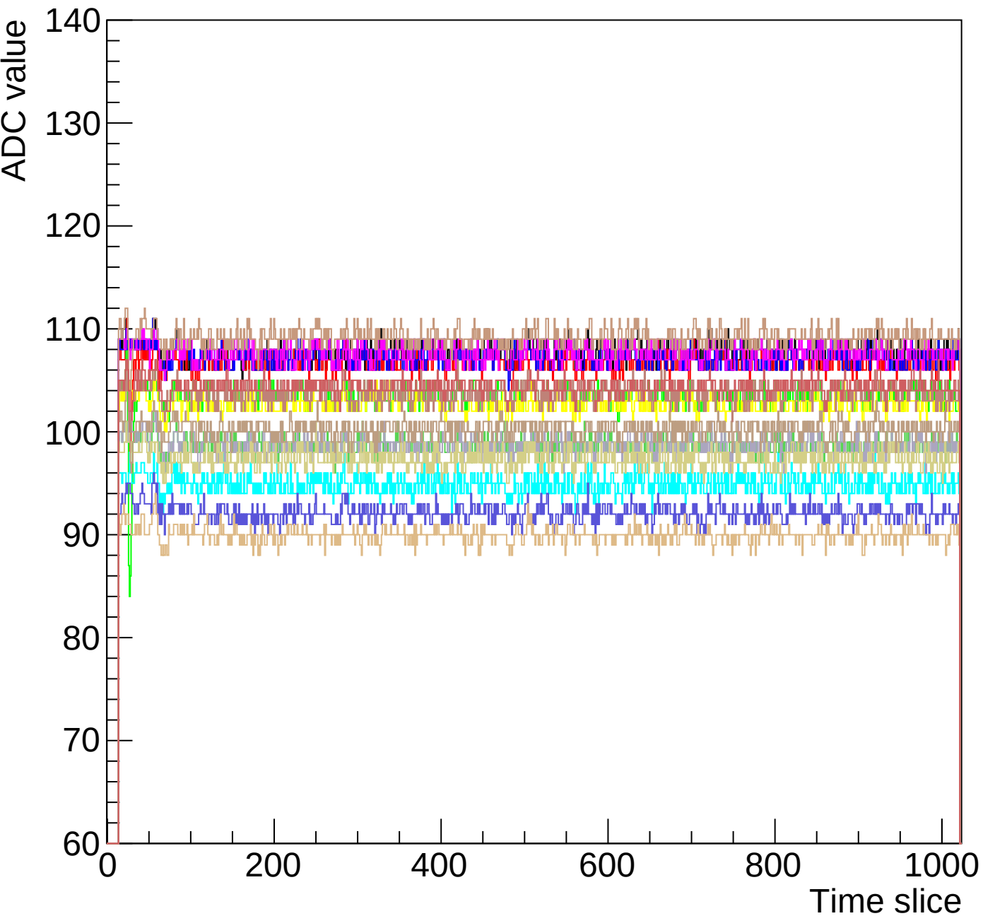
Run 0 event 20 mcm 0 chip 4 chamber-fec01-debug1
